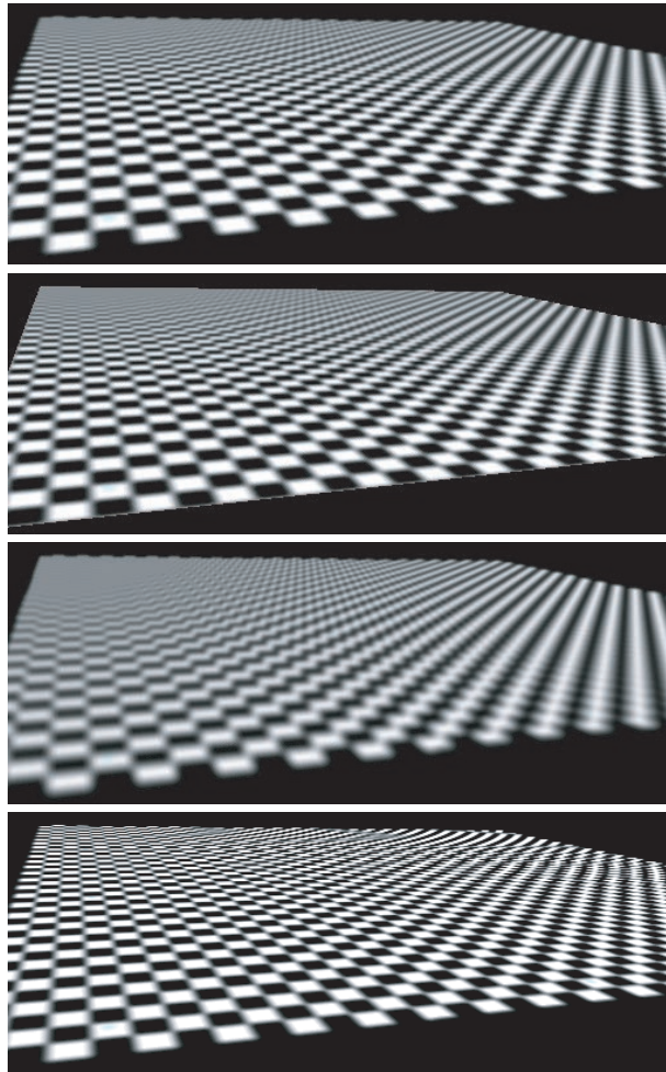
Figure 8: Top row: screen space EWA. Second row: source space EWA. Third row: circular splats. Bottom: elliptical splats.
