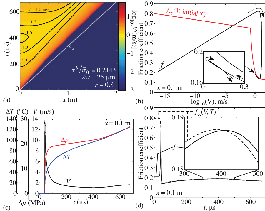
Figure C2. A crack-like solution accounting for changes in T and p due to shear heating. (a) Evolution of V . Slip acceleration occurs in the central region of the rupture. The white lines show contours for V = 1.0, 1.2, and 1.5 m/s. Contours at the rupture tip are not plotted. (b) A trajectory of (V, f) at x = 0.1 m reverses in the high- V and low- f direction (indicating the transition to a crack-like solution). (c) Time history of V, T, and p at x = 0.1 m. T and p keep increasing after the transition to a crack-like solution. (d) Time history of f and f_{ss}(V, T) . At the transition to a crack-like solution, f becomes larger than f_{ss}(V, T) .
