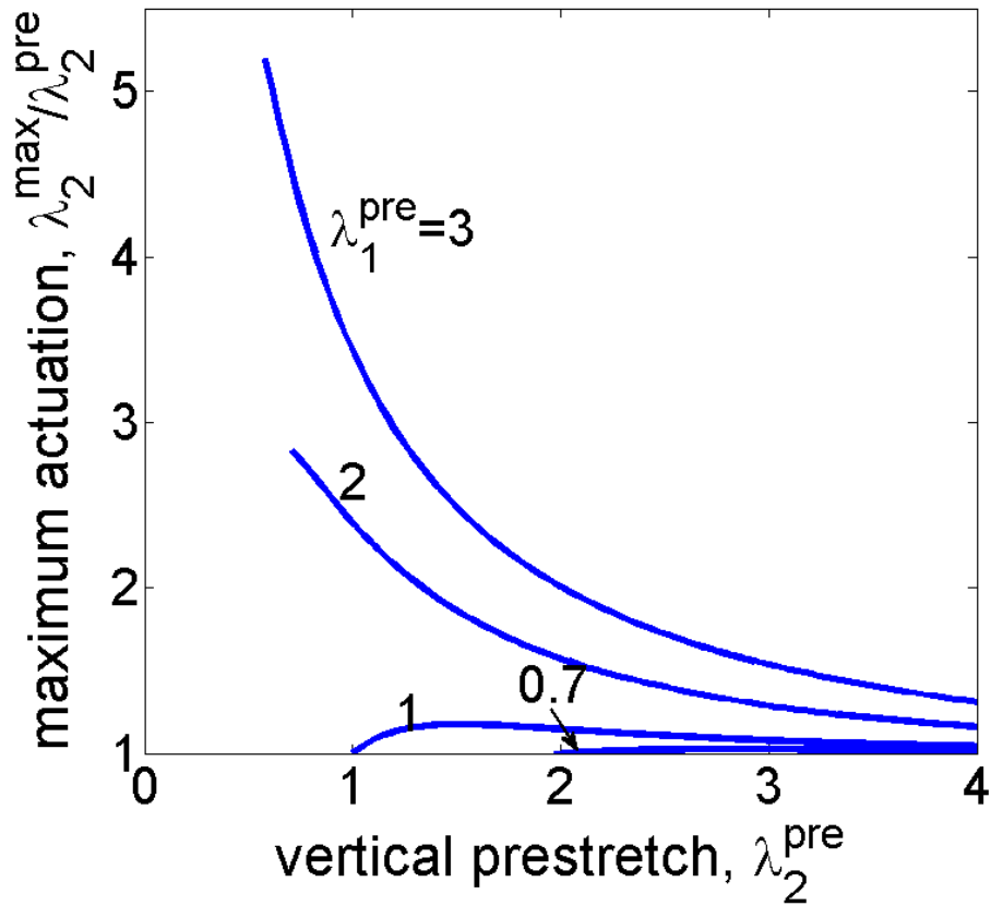
Fig. 6 Maximum actuation of a fiber-constrained membrane. The maximum actuation \lambda_2^{\max} / \lambda_2^{pre} is plotted as a function of the vertical prestretch \lambda_2^{pre} for several values of the horizontal prestretch \lambda_1^{pre} .
