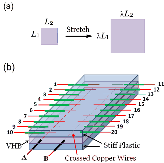
FIG.1 (Color online) (a) An elastomer sheet is stretched biaxially by an amount denoted as the stretch ratio \lambda ; (b) Electrical test arrangement consists of a prestretched elastomer sheet with an array of parallel cylindrical wires on either side, all embedded by casting a stiff polymer around them. The polymer blocks on either side of the elastomer sheet were made from a two component polyurethane mixture that, once cross-linking had initiated, was cast around the stretched elastomer to form a stiff plastic layer about 3 mm in thickness after fully curing. The electrodes consisted of high purity (99.99%) copper wires with a diameter of 18 \mu m encapsulated in the stiff polymer on either side of the elastomer are arranged at right angles to one another. Electrical connection was made to the individual wires, allowing for a large number of individual tests to be made on the same sheet. For example, 20 tests can be made in the configuration shown in the schematic.
