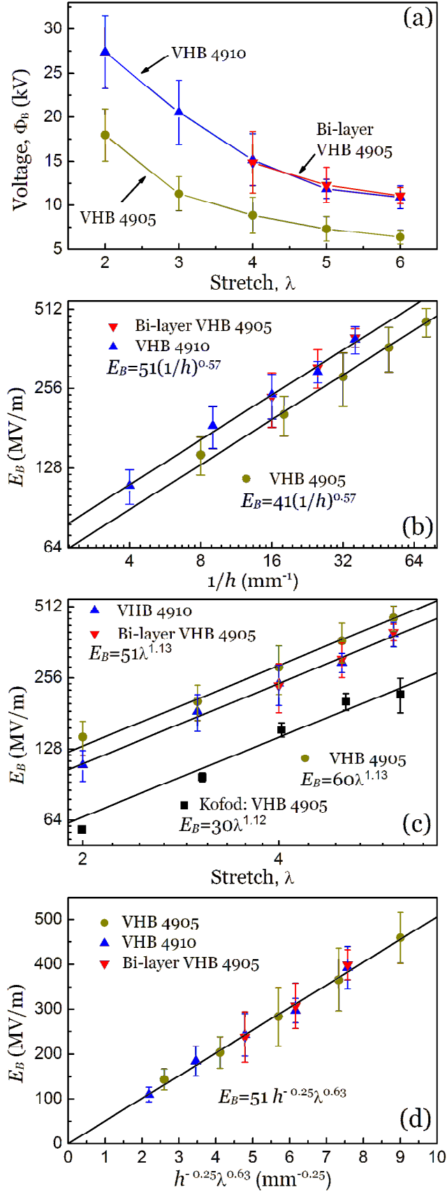
FIG.2 (Color online) (a) For each initial dielectric thickness, the breakdown voltages decrease monotonically with increase of stretch. (b) Breakdown electric field as a function of thickness for VHB 4905, two-layer VHB 4905 and VHB 4910 stretched to the values
