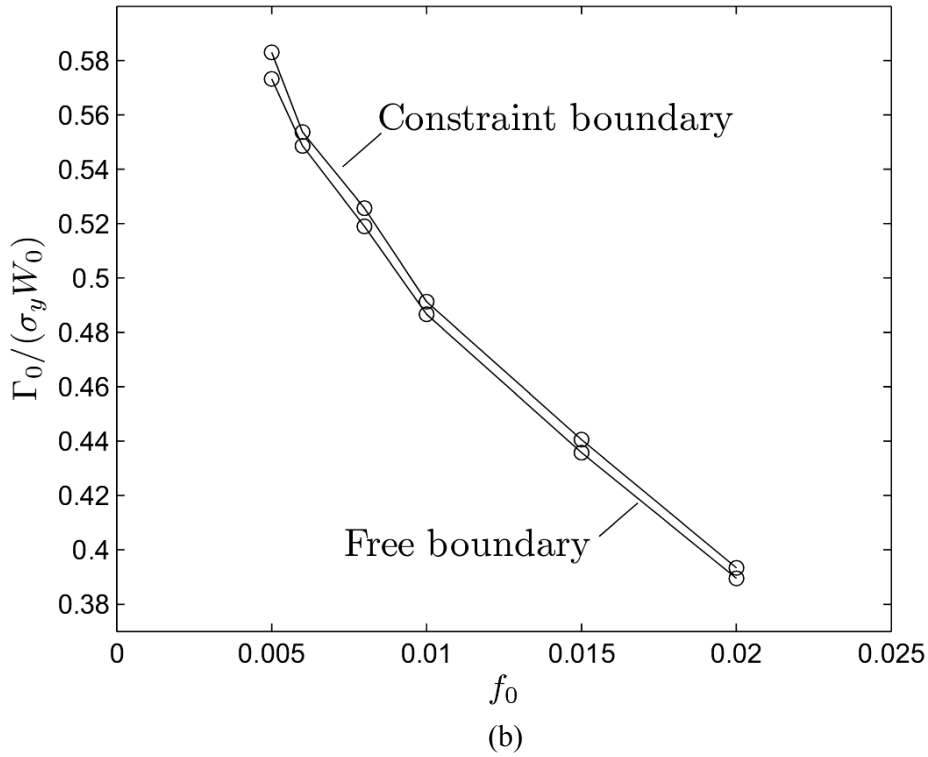
Figure 6: Effect of the out-of-plane deflection constraint across the fracture zone: (a) normalized overall load-deflection curves for constrained and unconstrained sections and (b) associated cohesive energy, \Gamma_0 = \Gamma_I + \Gamma_{II} , for f_0 \in [0.005, 0.02] , N = 0.1 , k_o = 0 and \sigma_y / E = 0.003 .
