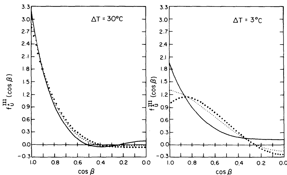
FIG. 15. Plots of the theoretical and experimental truncated angular distribution function f_{\frac{3}{2}}^{III}(\beta) : solid lines, HJL theory; large dots, Raman measurements from Fig. 13; small dots, estimation from Table I.
