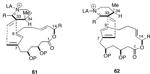
Figure 3.9 Dr. Chiu's concept for macrocyclic dienes.
