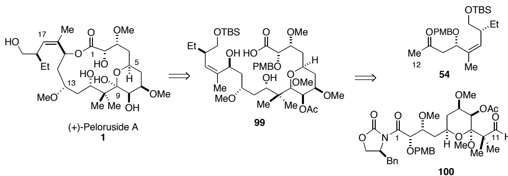
Figure 1.16 The first generation synthesis plan.
