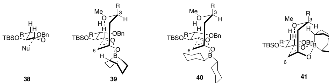
Figure 2.4 Possible transition states for the C 6 -C 7 bond construction.
