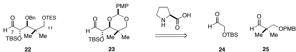
Figure 2.3 Redesigned C 7 –C 11 fragments
