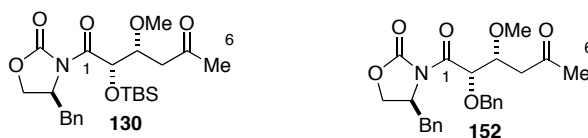
Figure 1.18 Methyl ketones utilized by Dr. Welch.
