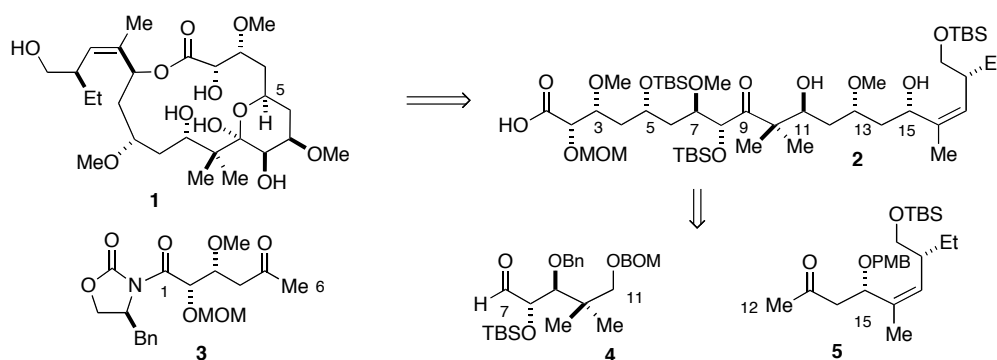
Figure 2.1 Fragments targeted in this work.
