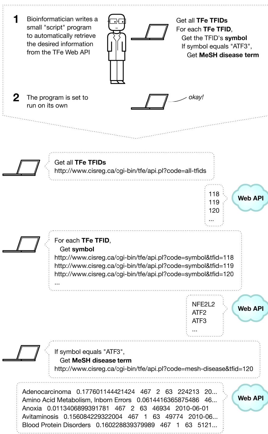
Figure 9 Using the TFe web API. Adventures in bioinformatics often involve large amounts of data retrieval and computation not amenable to manual labor. Thus, in place of humans, software is written to automate the grunt work, which may include computing vast quantities of data or obtaining large amounts of information from resources in the cloud, such as NCBI. To give researchers the option to retrieve data from TFe in an automated fashion, we have implemented a simple yet powerful web API. This figure provides a summary of what a data transaction may look like when using the TFe web API. In this case, the goal of the data retrieval exercise is to obtain all MeSH disease terms associated with the transcription factor 'ATF3'.
