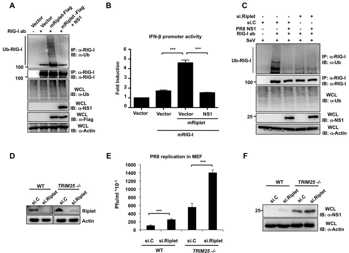
Figure 7. NS1 inhibits the Rippet-dependent RIG-I ubiquitination and IFN induction in murine cells. (A) Mouse Hepa 1.6 cells were transfected with vector or Flag-tagged mRippet with or without NS1-PR8. WCLs were subjected to IP with RIG-I antibody, followed by IB with anti-Ub or anti-RIG-I antibody. Expression of mRippet, NS1, and ubiquitin (Ub) was determined in the WCLs by IB with anti-Flag, anti-NS1 or anti-Ub antibody. (B) Mouse Hepa1.6 cells were transfected with IFN- \beta luciferase reporter plasmid together with empty vector or mRIG-I together with or without mRippet and NS1-PR8. At 24 h posttransfection, cells were lysed and subjected to luciferase assay. Data shown is representative of 3 independent experiments and depicted is the mean \pm SD ( n = 3 ). (C) Influenza NS1 protein specifically inhibits the Rippet-dependent ubiquitination of mouse RIG-I. Hepa1.6 cells were transiently transfected with non-silencing control siRNA (si.C), or with a siRNA specific for mouse Rippet (si.Rippet) together with empty vector or NS1-PR8. At 24 h posttransfection, cells were infected with SeV (50 HA units/ml) for 22 h. WCLs were used for IP with anti-RIG-I antibody, followed by IB with anti-Ub or anti-RIG-I antibody. (D–F) Knockdown of endogenous Rippet in mouse embryonic fibroblasts enhances influenza A virus replication. WT or TRIM25 -/- MEFs were transfected with non-silencing control siRNA (si.C), or with a siRNA specific for mouse Rippet (si.Rippet). At 30 h posttransfection, cells were infected with recombinant A/PR/8/34 WT virus (MOI 0.1). Knockdown of endogenous Rippet was confirmed by RT-PCR (D). Supernatants were assayed for progeny virus yields 24 h postinfection in standard plaque titrations (E). Virus yields are depicted in Pfu/ml. The results of three independent experiments are shown. Furthermore, viral NS1 protein expression was determined in the WCLs of infected cells (F). doi:10.1371/journal.ppat.1003059.g007
