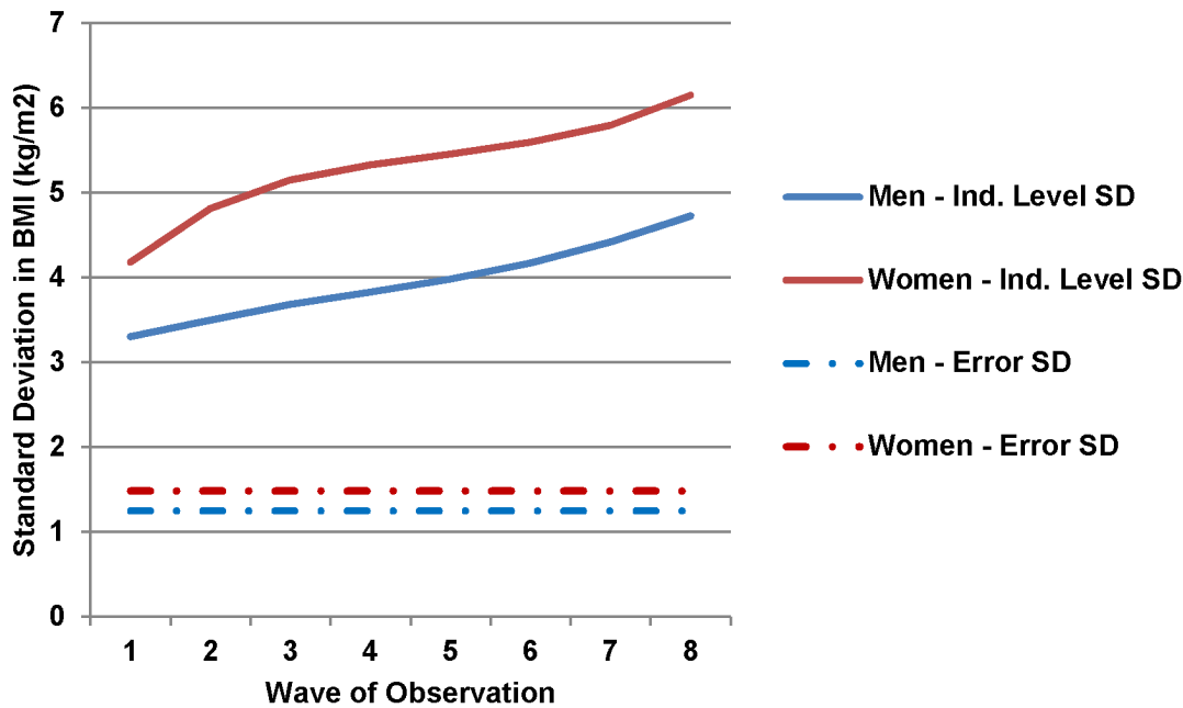
Figure 2. Adjusted Standard Deviation in Body Mass Index, Framingham Heart Study Offspring Cohort, 1971–2008. In the fully adjusted models, the total unexplained variation in BMI attributed to individuals across time (individual-level standard deviation) steadily increased from 1971 to 2008 for both women and men. The error standard deviation represents the idiosyncratic pure error variance. We accounted for non-linear increases in between-individual BMI standard deviation by including a random intercept at the individual level and random slopes for time and the natural log of time. doi:10.1371/journal.pone.0063217.g002
