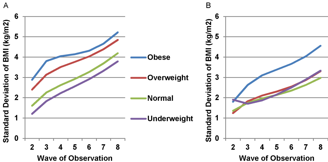
Figure 4. Individual-Level Standard Deviation in Body Mass Index by Baseline Weight Classification, Framingham Heart Study Offspring Cohort, 1979–2008. In the fully adjusted models, the individual-level standard deviation of BMI steadily increased from 1971 to 2008 for both women (A) and men (B) in all baseline weight classifications. Standard deviation increases were similar across most weight classifications with larger standard deviations for both obese women and men, and larger increases across time for obese men. We accounted for non-linear increases in between-individual BMI standard deviation by including a random intercept at the individual level and random slopes for time and the natural log of time.
