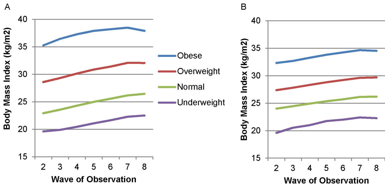
Figure 3. Body Mass Index Trajectories by Baseline Weight Classification, Framingham Heart Study Offspring Cohort, 1979–2008. Using results from the fully-adjusted models, we plotted the BMI trajectory for women (A) and men (B) based on their weight classification at baseline (during Wave 1, 1971–1975), controlling for covariates including baseline BMI. Weight classifications were underweight (BMI <18.5 kg/m 2 ), normal weight (18.5 to 24.9), overweight (25 to 29.9), and obese (≥30). Lines represent trajectories for the typical male or female (mean age at each wave, married, employed, >high school education, non-smoker, consuming 1–2 alcoholic drinks daily, living in a census tract at mean poverty level, with mean baseline BMI for that weight classification). doi:10.1371/journal.pone.0063217.g003
