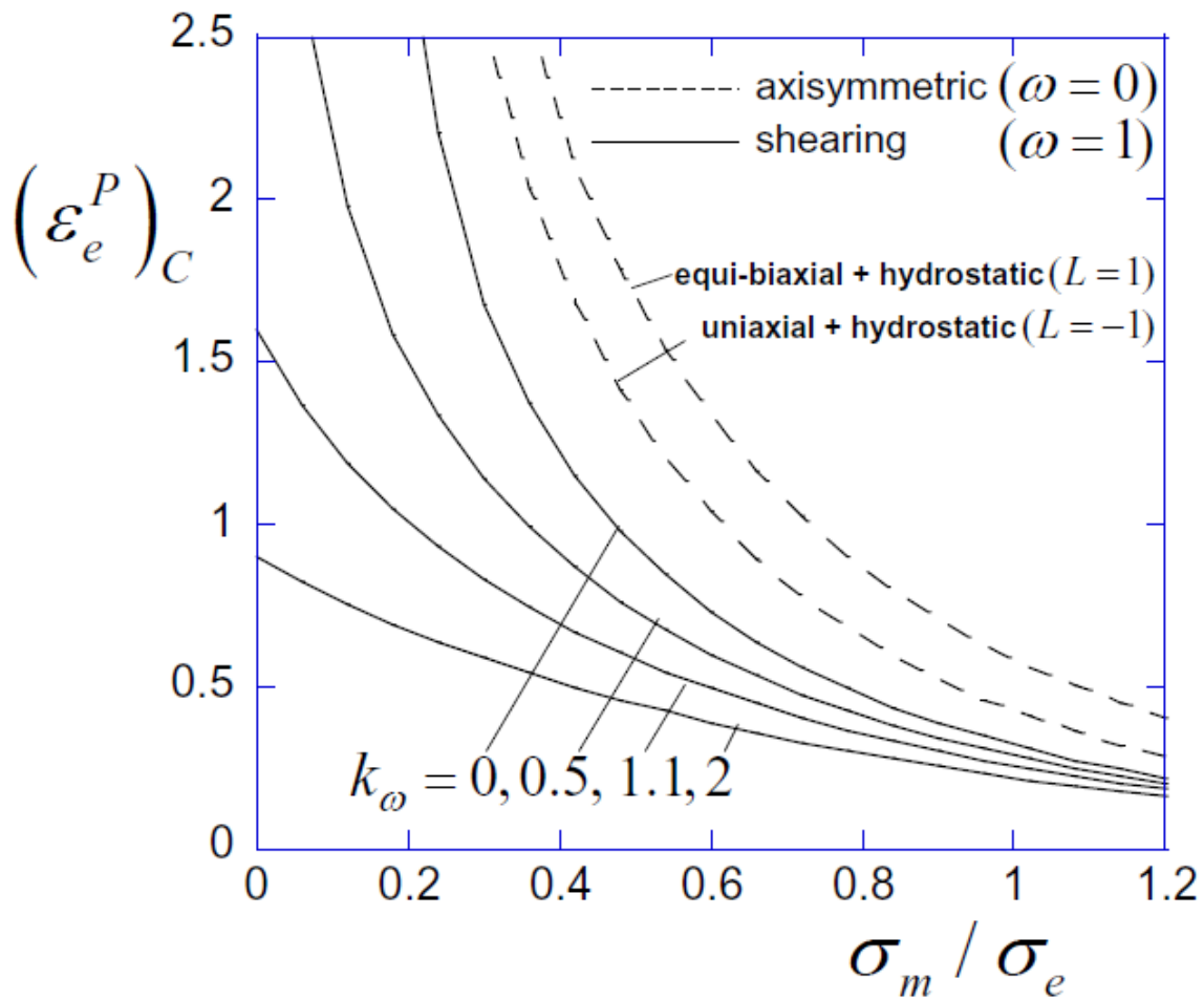
Fig. 2 Critical effective plastic strain at localization as a function of triaxiality for axisymmetric stressing and shearing stress states with f_0 = 0.005 inside the band. The results for axisymmetric stressing are essentially independent of the shear damage coefficient, k_\omega , while those for shear stressing depend strongly on k_\omega . The result for k_\omega = 0 is that based on the conventional Gurson Model. The result for k_\omega = 1.1 is that based on the extended model calibrated to Weldox 420.
