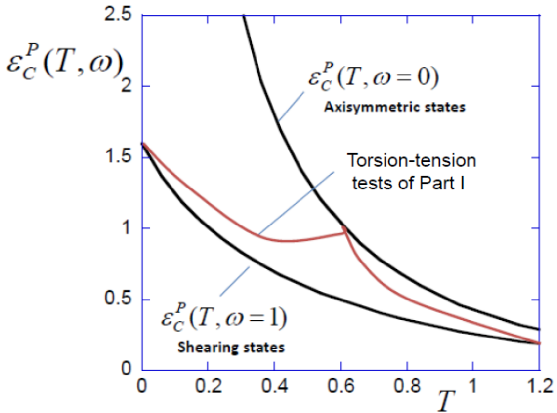
Fig. 16 A schematic plot illustrating the phenomenological critical strain criterion (15) showing the two bounding curves: the upper curve for axisymmetric stress states and the lower curve for shearing stress states. The schematic trend of the torsion-tension tests between these two limiting curves is also included.
