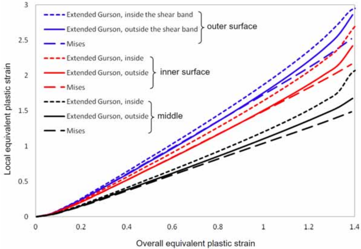
Fig. 13 The equivalent plastic strain at three locations within the minimum section of the notch as a function of the overall equivalent plastic strain for Weldox 420 for torsional loading ( k_T = 0 ). As noted in Fig. 12, for this loading the strains are larger at the outer and inner surfaces than at the middle of the notch. Three predictions are shown for each location: (1) based on Mises theory with no damage (i.e., f_0 = 0 ) using precisely the same mesh, based on the extended Gurson model within the incipient shear band (2), and just outside the incipient shear band (3). The strains within and outside the emerging shear band begin to diverge prior to the onset of failure in torsion at overall equivalent plastic strain slightly less than 1.4. The results for Mises plasticity with no damage are reasonably accurate until the overall strain approaches the onset of failure.
