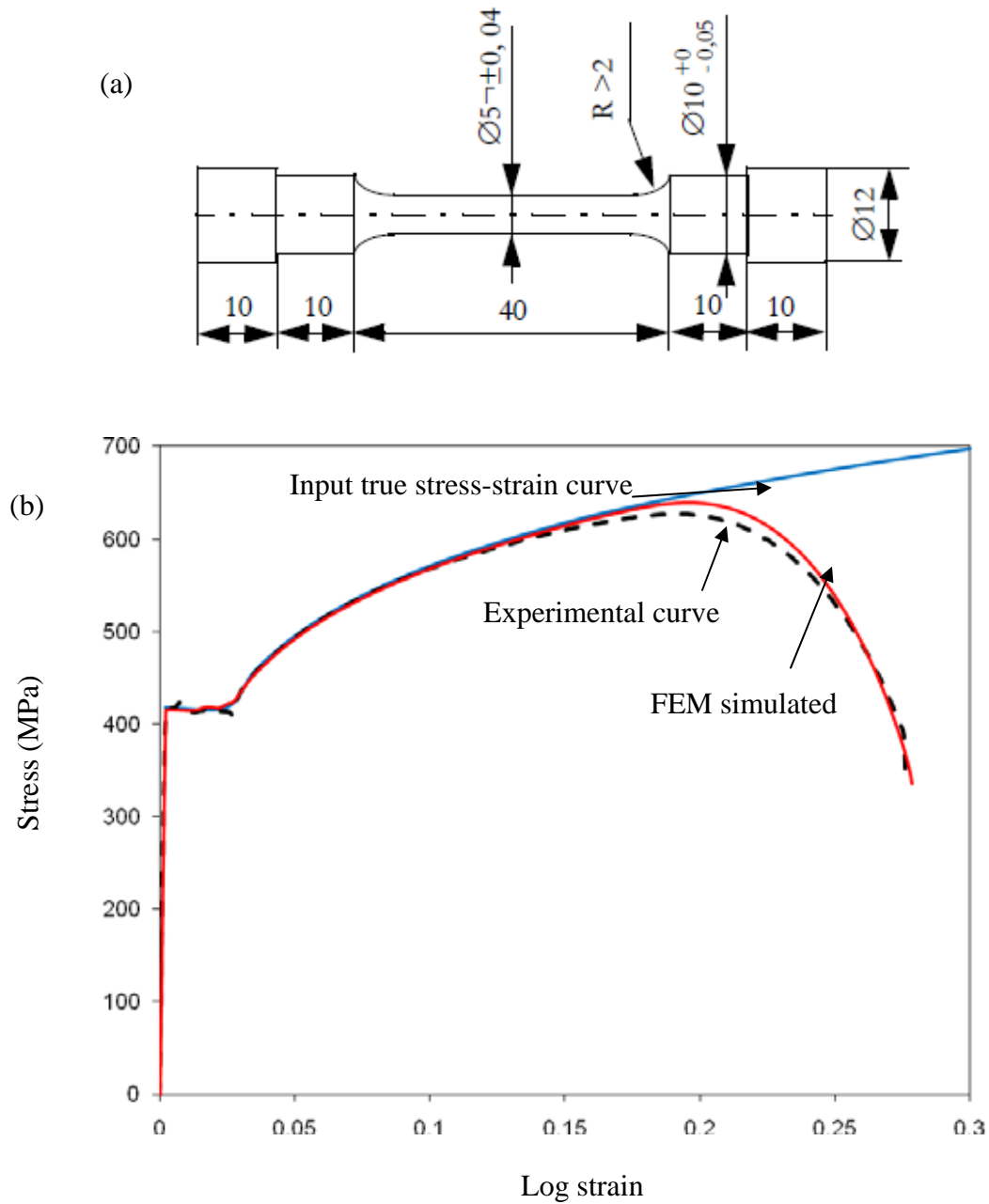
Fig. 5 (a) Dimensions of the round smooth bar specimen (in mm). (b) Stress-log strain curve for Weldox 420. For the experimental curve and FEM simulated curve, the stress plotted is determined as (P/A_0)(L/L_0) where P is the load, A_0 is the initial cross-sectional area of the gage section, and L/L_0 is the ratio of deformed to undeformed length of the gage section. The log strain is \ln(L/L_0) . The input curve is the true stress-log strain curve (13) with parameter values given in Table I.
