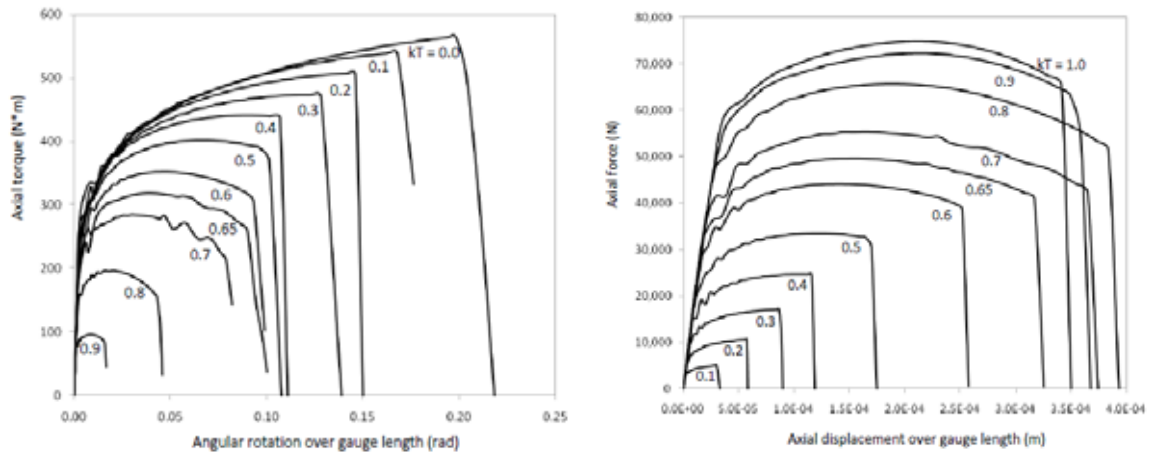
Fig. 9 Computed curves of torque versus rotation across the notch and axial force versus axial displacement across the notch for the series of tests, each with constant k_T , for Weldox 420.
