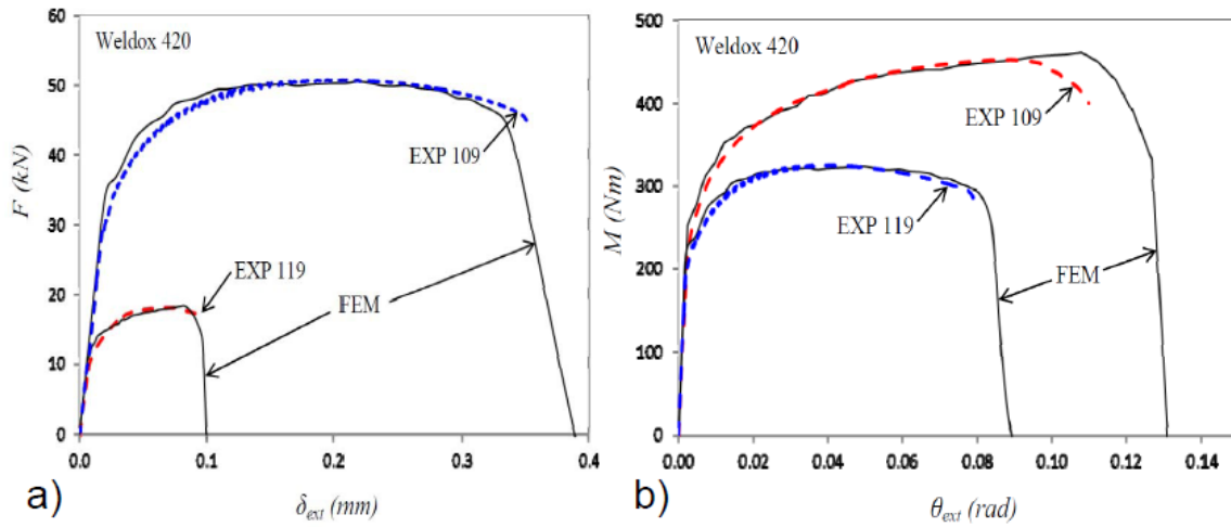
Fig. 10 Comparison of simulations with experimentally measured force-displacement relation in a) and moment-twist relation in b) for two of the experiments. Experiment 109 has k_T = 0.324 and experiment 119 has k_T = 0.651 .
