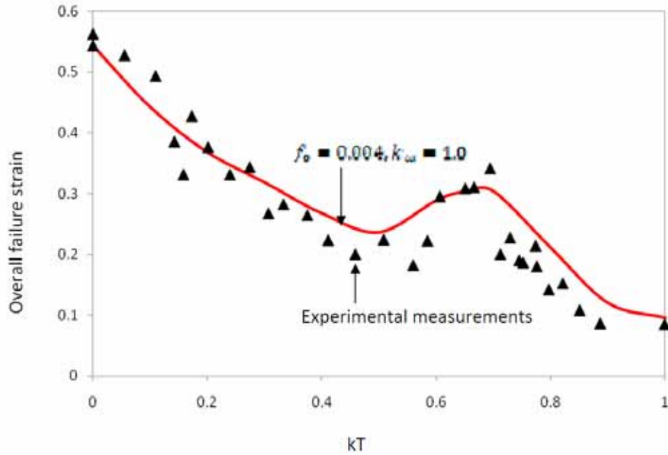
Fig. 14 A comparison of the experimental data for the tension-torsion tests for the high strength steel Weldox 960 with finite element simulation based the extended Gurson model. The overall plastic strain at fracture (defined in Part I) versus the relative proportion of tension to torsion as measured by k_T .
