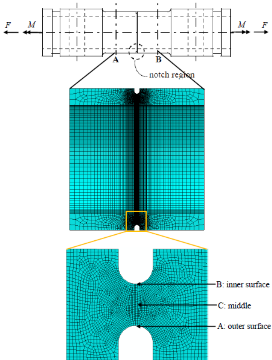
Fig. 8 The tension-torsion specimen and the finite element mesh used in the finite element analysis.
