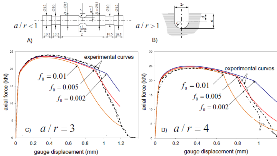
Fig. 6 Notched round bar tests used for calibrating the initial void volume fraction, f_0 . Specimen geometry in mm: A) a/r < 1 and B) a/r > 1 . Two tests for each of two notch geometries are shown along with simulations for several choices of f_0 : C) for a/r = 3 and D) for a/r = 4 .
