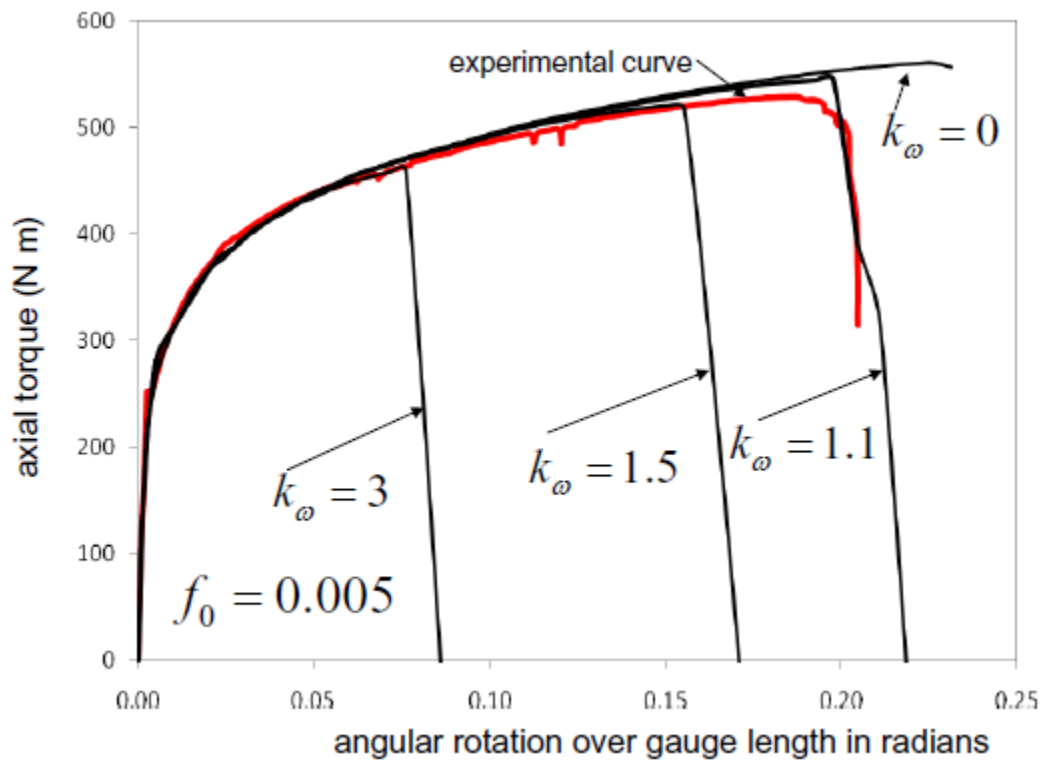
Fig. 7 Calibration of the shear damage coefficient, k_\omega . Experimental data from the pure torsion test of the tension-torsion series of Part I compared with simulations of the specimen for four values of k_\omega .
