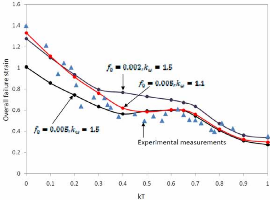
Fig. 11 A comparison of the experimental data for the tension-torsion tests for Weldox 420 with finite element simulation based the extended Gurson model. The overall plastic strain at fracture (defined in Part I) versus the relative proportion of tension to torsion as measured by k_T . The calibrated damage parameters for Weldox 420 are ( f_0 = 0.005, k_w = 1.1 ). Predictions for two other sets of damage parameters are show to give an indication of the sensitivity to these parameters.
