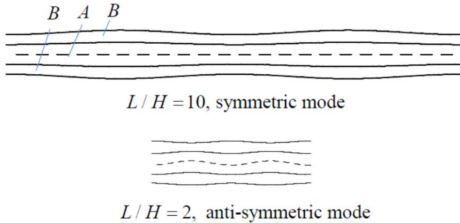
Fig. 4 The bifurcation mode shapes associated with Fig. 3b for the case of the weaker material in the central layer ( \sigma_0^A/\sigma_0^B = 0.05 ). The plots display the variation of the normal displacement increment, v_2 , for the layer boundaries (and the centerline, which is dashed) associated with the bifurcation mode. The sign and amplitude of the shape are arbitrary.
