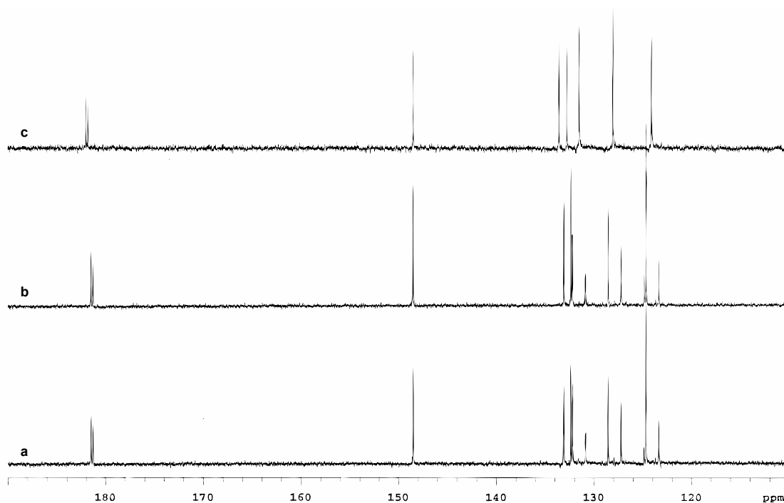
Extended Data Figure 6 | 13 C NMR (500 MHz, D 2 O) spectra. a , AQDS, \delta = 181.50 p.p.m. versus TMS (C 9), 181.30 p.p.m. (C 10), 148.51 p.p.m. (C 2,7), 133.16 p.p.m. (C 11), 132.40 p.p.m. (C 12), 130.86 p.p.m. (C 3,6), 128.59 p.p.m. (C 4,5), 124.72 p.p.m. (C 1,8). b , The same sample, 24 h after addition of Br 2 . c , 13 C NMR of AQDS treated with 2 M HBr and Br 2 and heated to 100 °C for 48 h.
