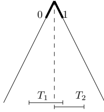
Fig. 1. Example of how a \text{SV}(\gamma) \in \mathcal{SV}(\gamma) distribution can increase the ratio \frac{\Pr_{\mathbf{r} \leftarrow \text{SV}(\gamma)}[\mathbf{r} \in T_1]}{\Pr_{\mathbf{r} \leftarrow \text{SV}(\gamma)}[\mathbf{r} \in T_2]} .
