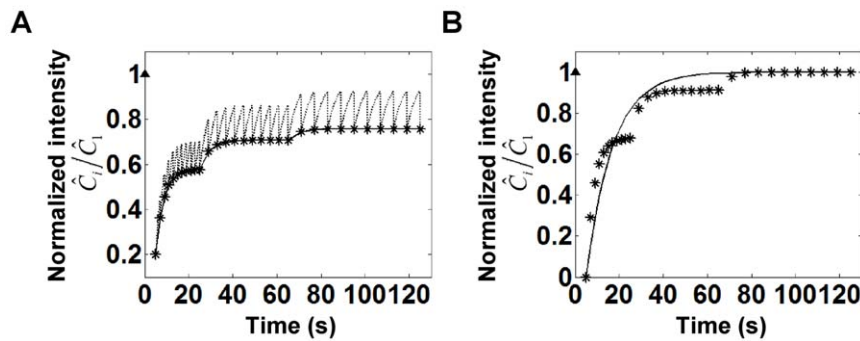
Figure 5. Predicted FRAP dynamics with changing time interval \tau . (A) Recovery curve calculated from Eq. 6 with parameters k_{OFF} = 0.2 , \alpha = 0.2 , \lambda\omega = 0.2 , \tau = 2s, 4s, 6s ( \tau increased after every 10 images). The dotted curves show the predicted unobserved dynamics. (B) Fitting of \frac{\hat{C}(t) - \alpha\hat{C}_1}{\hat{C}_\infty - \alpha\hat{C}_1} = 1 - e^{-tk_{OFF}} to the normalized predicted data from A. The fitting yields k_{OFF} = 0.0846 , much different from the actual value of k_{OFF} = 0.2 . doi:10.1371/journal.pone.0042854.g005
