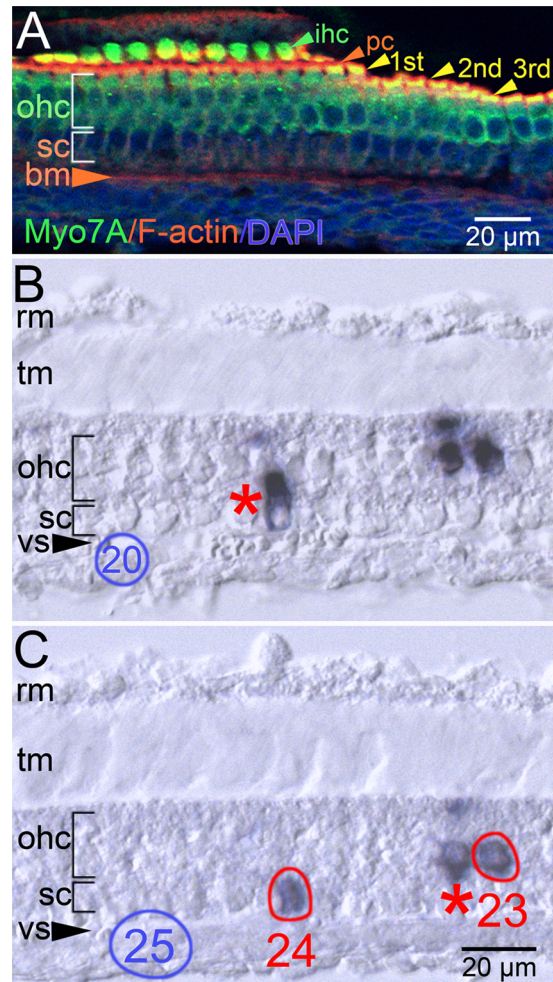
Figure 4. Outer hair cells and a supporting cell type are clonally related. A, confocal projection of an oblique, 14 \mu\text{m} section of a control P6 cochlear duct. Sensory hair cells (myosin7a [Myo7A], green), filamentous actin (F-actin, red), and cell nuclei (DAPI, blue) are detectable in this atypical histological presentation of the organ of Corti. The Myo7A-positive inner hair cells (ihc) are separated from the 1 st , 2 nd , and 3 rd rows of Myo7a-positive outer hair cells (ohc, wide bracket) by the F-actin-enriched apices of pillar cells (pc). The supporting cell (sc) nuclei occupy a region beneath the Myo7a-positive outer hair cells (ohc) indicated by the narrow bracket. B, C, oblique, 14 \mu\text{m} , serial cryostat sections of a P6 organ of Corti in a similar orientation as in panel A presenting PLAP-positive cells of a clone. The supporting cell in pick 24 and the outer hair cell in pick 23 returned the identical sequence tag. The supporting cell in panel B (red asterisk) and the hair cell in panel C (red asterisk) did not return an oligonucleotide sequence. Negative control picks 20 (blue oval, panel B) and 25 (blue oval, panel C) did not generate a PCR product. The atypical plane of section precludes clear identification of the supporting cell type in the ohc clone. Abbreviations: bm, basilar membrane; rm, Reissner's membrane; tm, tectorial membrane; vs, vas spirale (tangential section).
