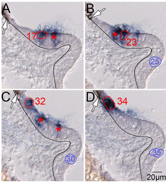
Figure 3. Sensory hair cells and nonsensory epithelial cells of the posterior crista are clonally related. A–D, serial, 14 \mu\text{m} sections of the posterior crista demonstrating the PLAP-positive constituents of a mixed sensory/nonsensory epithelial clone. The black line demarcates the boundary between the sensory epithelium (right) and the underlying mesenchyme (left) of the crista ampullaris. The red ovals are picks of PLAP-positive cells that returned the identical sequence tag. Picks 17 and 23 are in the hair cell layer of the crista while picks 32 and 34 are proximal to neural crest-derived melanocytes (white arrows) in the adjacent, nonsensory epithelium (see also Fig. 1, panel D, left, white arrow). The blue ovals (25, 30, and 35) are control picks of PLAP-negative tissue that did not generate a PCR product. The red asterisks indicate location of PLAP-positive cell picks that failed to return a PCR product.
