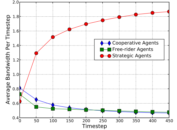
Figure 5: Bandwidth in BarterCast Mechanism over Time.
