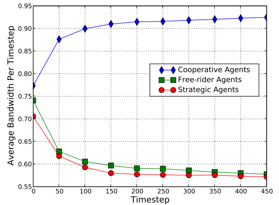
Figure 6: Bandwidth in Drop-Edge Mechanism over Time.
