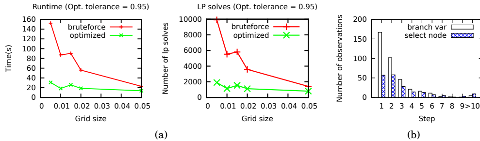
Fig. 8. (a) Runtime and number of LP solves for brute force and optimized ironing procedures. (b) Histogram of the steps at which search decisions change, for different change types. \gamma = 0.95, \beta = 0.01 , averaged over all bucket sizes and datasets. 300 agents, 30 items.
