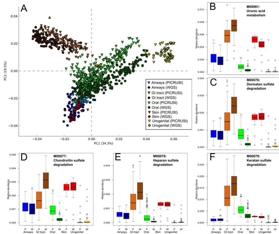
Figure 2. PICRUSt recapitulates biological findings from the Human Microbiome Project. A) PCA plot comparing KEGG Module predictions using 16S data with PICRUSt (lighter colored triangles) and sequenced shotgun metagenome (darker colored circles) along with relative abundances for five specific KEGG Modules, B) M00061: Uronic acid metabolism, C) M00076: Dermatan sulfate degradation, D) M00077: Chondroitin sulfate degradation, E) M00078: Heparan sulfate degradation, and F) M00079: Keratan sulfate degradation, all involved in glycosaminoglycan degradation (KEGG pathway ko00531) using 16S with PICRUSt (P, lighter colored) and WGS (W, darker colored) across human body sites: nasal (blue), gastrointestinal tract (brown), oral (green), skin (red), and vaginal (yellow).
