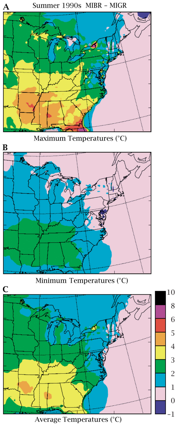
Fig. 3. Differences in simulated surface temperatures, MIBR minus MIGR, for JJA 1993–1997: (A) maximum temperatures; (B) minimum temperatures; (C) mean temperatures
