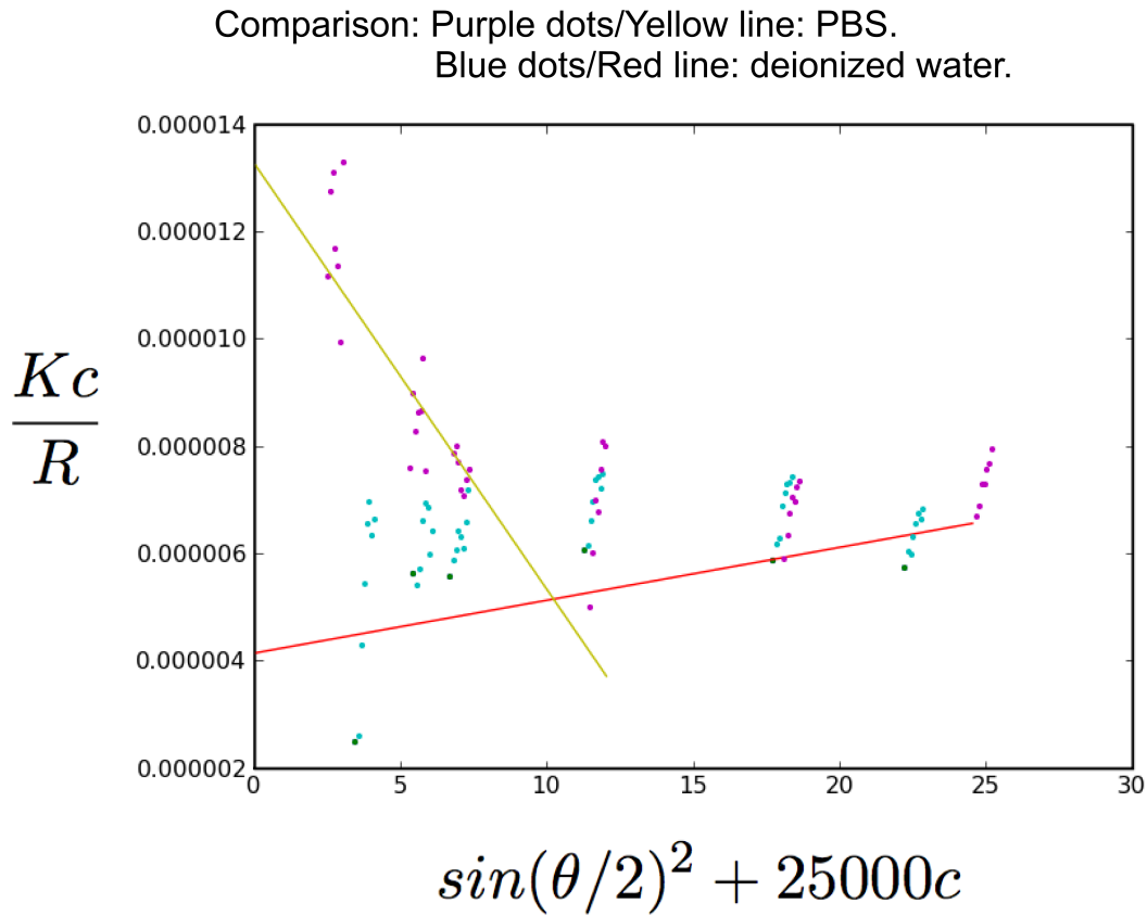
Figure 2.3: Dscam Isoform 1.30.34 IgG1-8 light scattering data. Each cluster of points corresponds to data taken at one concentration and various angles (45-120°). \frac{Kc}{R} \propto \frac{1}{I} . Low scattered intensity suggests monomers, and high intensity suggests dimers.
