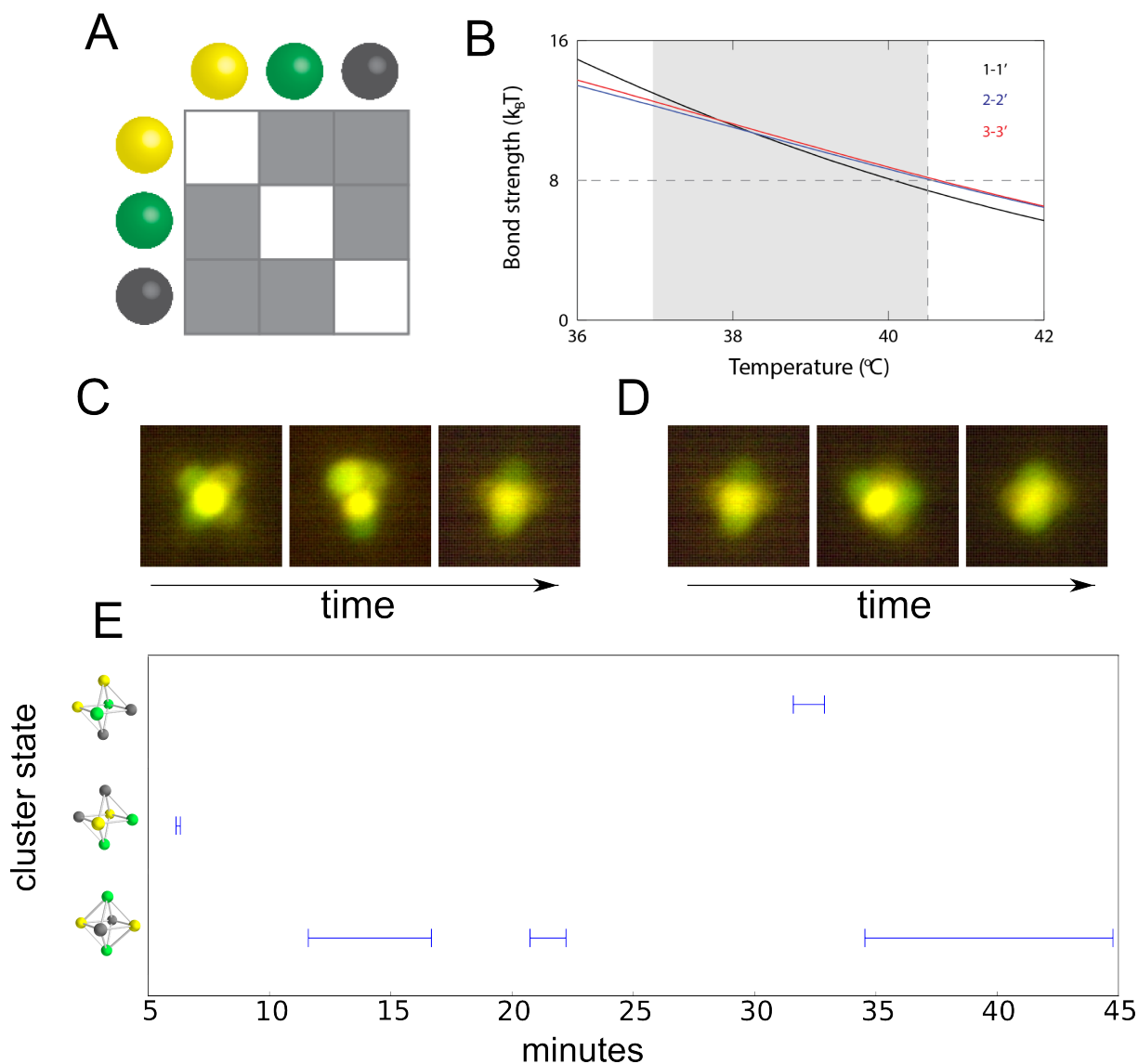
Figure 4.3: Specific, Equilibrium Interactions. A) Interaction Matrix. Particles of each type (color) bind only particles of a different type (color). Gray squares indicate favorable interactions, white indicates purely repulsive interactions. B) Bond strength versus temperature calculated from measured singlet fractions for each pair of attractive species. C) As might be expected for equilibrium binding, a cluster loses at least one green-yellow contact and transitions from one locally stable state to another over 6 minutes. D) The same cluster in C) loses a green-gray contact but regains it over 3 minutes. E) As bonds break and form, particles explore various configurations, as expected for equilibrium binding of a system with multiple stable energy-minimizing states. Panels A and B courtesy of W. Ben Rogers.
