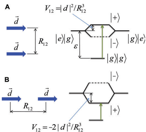
Figure 6 Interaction between electronic transition dipoles (blue arrows) of two molecules. The directions of the arrows reflect the relative phase of the transition dipoles. For the considered molecular alignments only one of the optical transitions is allowed for the dimer (green arrows). (A) The optically allowed transition of the dimer is shifted to the blue part of the spectrum, which is similar to H-aggregation; (B) the optically allowed transition is shifted to the red, which correspond to J-aggregation.
