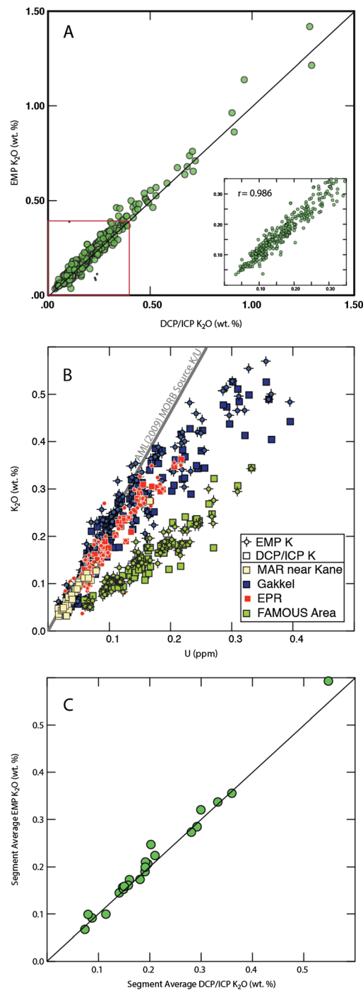
Figure 10. (A) Comparison of K 2 O measured by EMP to K 2 O measured by higher-precision techniques including DCP and ICP-MS in the Langmuir laboratory. Over a wide range of K 2 O contents, the measured values are remarkably coherent (with the exception of four samples, shown as small black squares, that were likely mislabeled). A 1:1 line is shown for reference. Inset shows depleted K 2 O values from 0 to 0.35, which are characterized by an R-value of 0.986. (B) K 2 O (measured by EMP and DCP or ICP-MS) versus U for samples from a wide geographic range measured in the Langmuir laboratory. Note that regional differences in K/U are captured whether K 2 O is measured by EMP or DCP/ICP. For reference, the K/U ratio estimated by AML [2009] for the “MORB Source” is shown. Note that the AML [2009] ratio is at the very depleted end of the MORB spectrum and is not representative of the mean MORB source. (C) Comparison of mean K 2 O calculated using EMP data versus mean K 2 O calculated using DCP or ICP-MS data for 23 ridge segments containing samples with K 2 O measured by both techniques in the Langmuir laboratory. Also shown is a 1:1 line for reference. Note how coherent the calculated mean K 2 O values are using both techniques, with 19 of 23 segment values agreeing to better than 9%.
