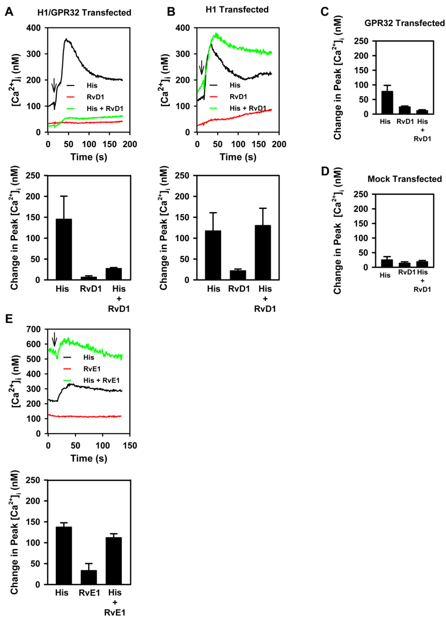
Figure 9. RvD1 uses the GPR32 receptor to block histamine activation of the H 1 receptor by phosphorylating the H 1 receptor in CHO cells A–D represent response of [Ca^{2+}]_i to histamine ( 10^{-5} M), RvD1 ( 10^{-8} M), or 30-min RvD1 exposure followed by histamine in fura-2 loaded CHO cells that had been transiently transfected with A. H 1 and GPR32 receptors, B. H 1 receptor, alone C. the GPR32 receptor alone, or D. mock transfected. A. and B. indicate intracellular [Ca^{2+}]_i over time (upper panels) or peak [Ca^{2+}]_i (lower panels) in response to histamine ( 10^{-5} M), RvD1 ( 10^{-8} M), or addition of RvD1 30 min before addition of histamine. C. and D. show peak [Ca^{2+}]_i in response to histamine, RvD1, or addition of RvD1 30 min before addition of histamine. E indicates intracellular [Ca^{2+}]_i over time (upper panel) or peak [Ca^{2+}]_i (lower panel) in response to histamine ( 10^{-5} M), RvE1 ( 10^{-8} M), or addition of RvE1 30 min before addition of histamine.
