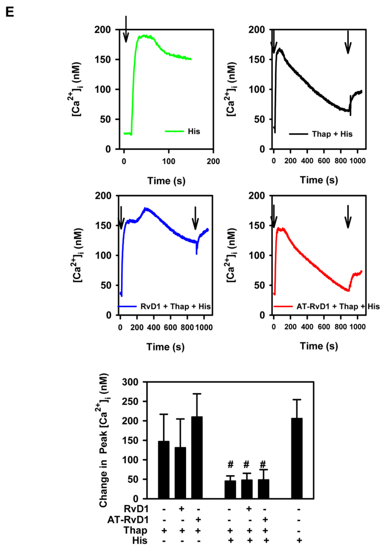
Figure 2. RvD1 and AT-RvD1 reduce histamine-stimulated increase in [Ca^{2+}]_i by preventing release of intracellular Ca^{2+} in conjunctival goblet cells
