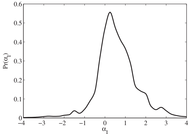
Figure 6. Source total intensity spectral index distribution Pr(\alpha_l) .
