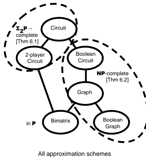
Figure 4: Summary of \text{EXISTSPURENASH} Results
