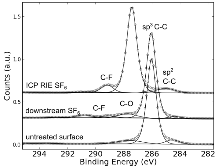
Figure 4.12: High resolution carbon scan of a diamond cleaned with boiling triacid, and fluorine-terminated with SF 6 in either a downstream reactor or an ICP RIE reactor. The sample etched in a ICP RIE has a significantly shifted main peak, which is likely due to lattice damage from the etch.
