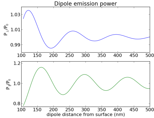
Figure A.2: Analytical solution to the total emitted power of a dipole, when z_0 > \lambda_1 .
