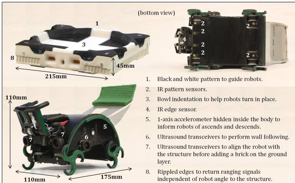
Figure 4.3.e. Features and sensors on robots and bricks enabling multiple robots to perform autonomous navigation reliably on and off the structure.
