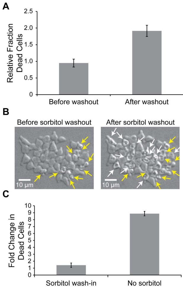
Figure 5. Phormone-induced cell death is due to osmotic lysis. A. MATa bar1Δ cells were grown in a flow chamber for five hours in medium with 50nM \alpha -factor and 1M sorbitol. After five hours, the sorbitol was washed out, and the cells were incubated in medium with 50nM \alpha -factor and no sorbitol. The fraction of dead cells 10 minutes before and 10 minutes after the 1M sorbitol was washed out relative to the fraction of cells that die when exposed to 50nM \alpha -factor for five hours without the addition of sorbitol was determined (Student's t -test, p=2\times 10^{-4} ). Error bars represent the standard deviation of at least three independent experiments. B. Cells imaged after 290 minutes in medium with 1M sorbitol and 50nM \alpha -factor (Before sorbitol washout) and 10 minutes after the medium was replaced with medium with 50nM \alpha -factor and no sorbitol (After sorbitol washout). Yellow arrows indicate the cells that died during the 290 minutes of phormone treatment prior to the sorbitol washout. White arrows in the "After sorbitol washout" picture indicate cells that died during the twenty minute period that spanned the last 10 minutes with sorbitol and the first 10 minutes after the sorbitol washout. The scale bar indicates 10 \mu m. C. Cells were grown in the flow chamber for 80 minutes in medium with 50nM \alpha -factor. After 80 minutes, 1M sorbitol was added to the medium such that the cells were incubated in medium with 1M sorbitol and 50nM \alpha -factor. The fold change in the number of cells that died during the 80 minutes prior to and 60 minutes after the sorbitol wash-in was determined (Sorbitol wash-in). In control chambers (No sorbitol), no sorbitol was added to the medium, and the fold change in the number of cells that died in the two corresponding periods was determined (Student's t -test, p=9\times 10^{-5} ). Error bars represent the standard deviation of at least three independent experiments. doi:10.1371/journal.pone.0109780.g005
