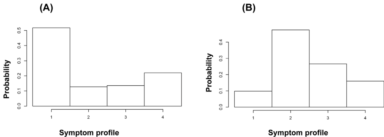
Figure 1. Distribution of symptom profiles for flu (A) and non-flu (B) symptomatic cases, inferred from data in [12] and [21]. Profile description is given in equation (2a). doi:10.1371/journal.pone.0023380.g001
