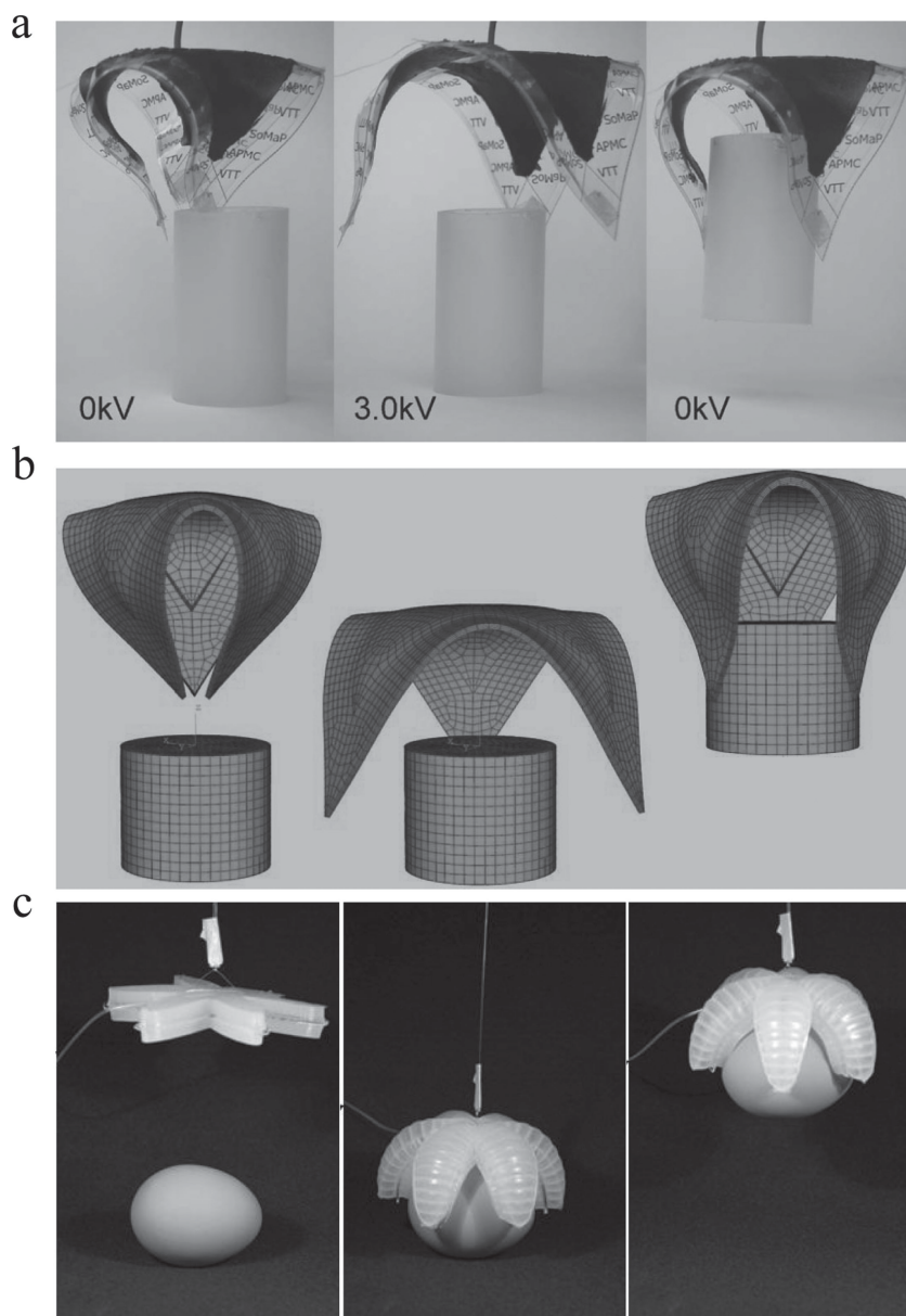
Figure 2. Grippers based on dielectric elastomers and PneuNets. (a) Dielectric elastomer actuator gripping a small Teflon cylinder. Reprinted with permission. [10] Copyright 2007, American Institute of Physics. (b) Finite element modelling of the dielectric elastomer actuator in (a). Reprinted with permission. [12a] Copyright 2008, American Institute of Physics. (c) PneuNet actuator gripping a raw egg. Reprinted with permission. [9a] Copyright 2011, Wiley-VCH.
