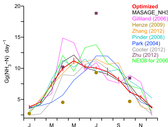
Figure 5. Estimates of total NH 3 emissions in the contiguous U.S. and their seasonal variation. Our optimized estimate from the adjoint inversion of NH 4 + wet deposition fluxes is compared to the MASAGE_NH3 bottom-up inventory (this work) and to previous estimates from the literature including bottom-up inventories (Park et al. [2004], Pinder et al. [2006], Cooter et al. [2012], and NEI08 ( http://www.epa.gov/ttnchie1/net/2008inventory.html )) and inverse analyses (Gilliland et al. [2006], Zhang et al. [2012], and Zhu et al. [2013]). The 2005–2008 interannual variability of our monthly optimized NH 3 emissions is indicated by red bars (one standard deviation). The GEOS-Chem a priori is based on Park et al. [2004].
