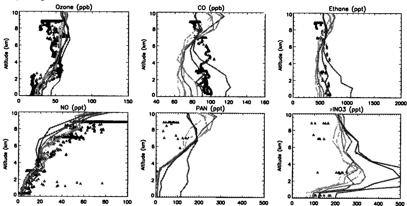
Figure 4. Comparison of model results with PEM-West B aircraft observations on (a) flight 17 and (b) flight 7 (see flight tracks in Figure 1). Triangles are observations. Grey lines are model results for the different grid squares along the flight track. The model values are 24-hour averages (daytime averages for NO) for the days of the flights.
