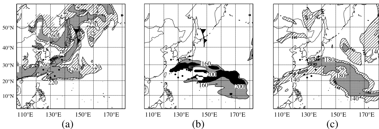
Figure 4. Simulated CO tracer, in ppbv, on 21 March 2001 at 0000 UTC (a) at 900 hPa, (b) on the 291 K wet-bulb potential temperature surface, and (c) at 300 hPa.
