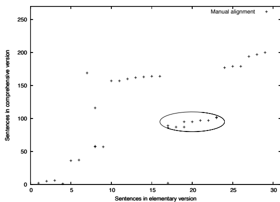
Figure 3: Gold alignment for a text from the Britannica corpus.
