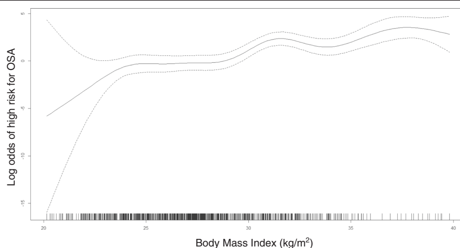
Fig. 1 Relation between log odds of high risk for obstructive sleep apnea and pre-pregnancy body mass index (solid line) with 95 % confidence interval (dotted lines)
