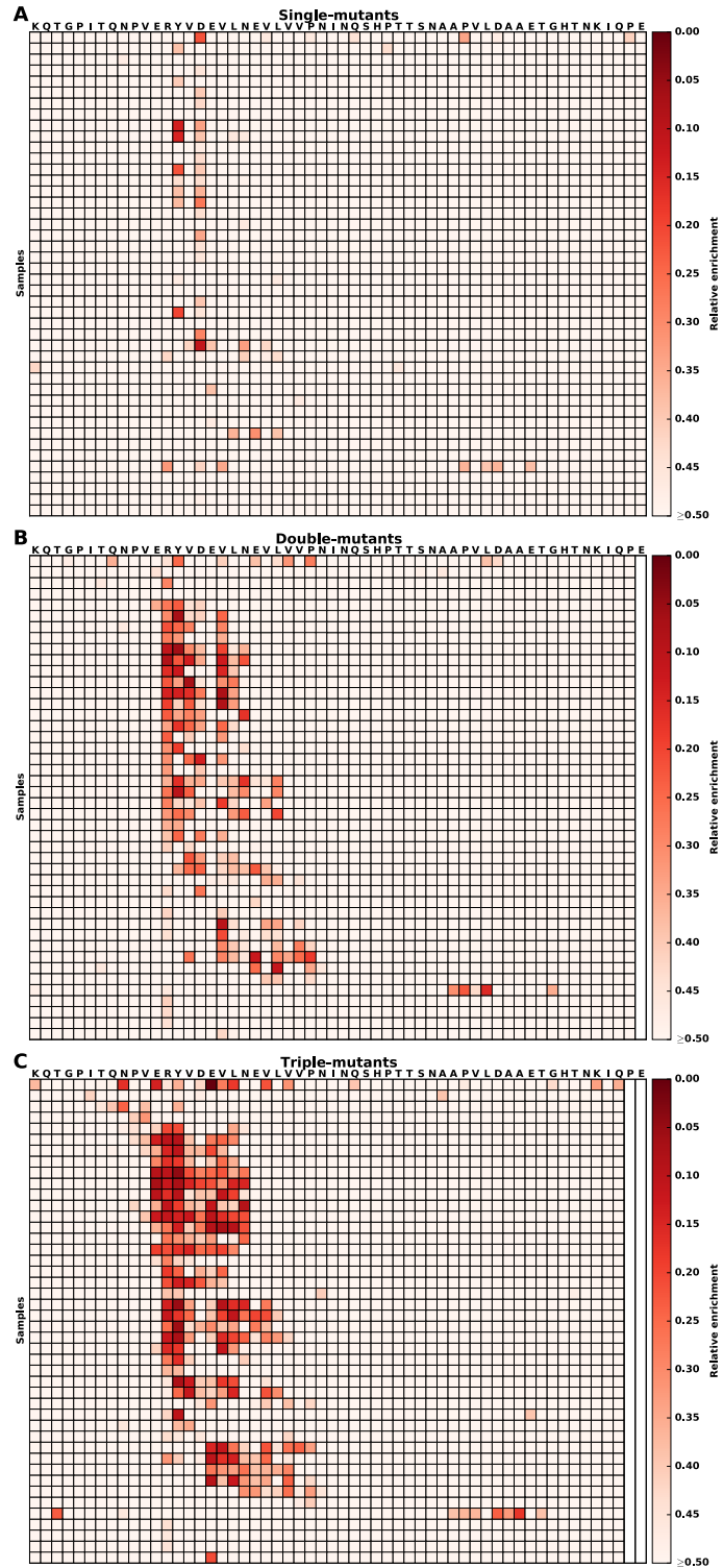
Figure 24. See caption for Figure 20. Rhinovirus A: genome polyprotein (UniProt ID: Q82122, positions 561-616)
