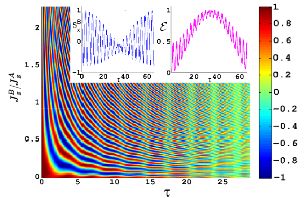
FIG. 5 (color online). Precession of qubit B starting at S_x^B = 1 in the geometry of Fig. 1(d). Qubit A is driven at its level splitting J_z^A with a Rabi frequency \epsilon = 0.3J_z^A , and qubit B is coupled to A with a coupling constant J_{AB} = 0.05J_z^A . Time \tau is in periods of the free precession of A . Color in the main panel and left inset: S_x^B(\tau) . Right inset: Entanglement \mathcal{E}(\tau) for J_z^B = 0.3J_z^A . See text for details.
