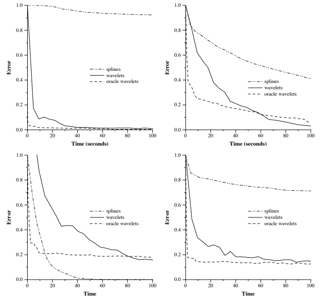
Figure 7: Error per time. Surface with 1089 control points, 11, 23, 64 evenly spaced constraints, and 62 constraints along the boundary.
