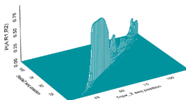
Figure 9. The structural alignment in (A) indicates that nearly all of the alignment between Inpx_2 and 3lada2 is conserved with two gaps. The SSEARCH optimal alignment (B) does not report the alignment of the first 34 residues of Inpx_2 and 26 residues of 3lada2 and incorrectly reports the remaining gap. This first section missed is a loop and thus is also missed by the alignment distribution of BALSAs (C). The alignment distribution clearly follows a similar pattern to that of the optimal but distinctly shows that there are many alignments similar to the optimal with comparative scores.
