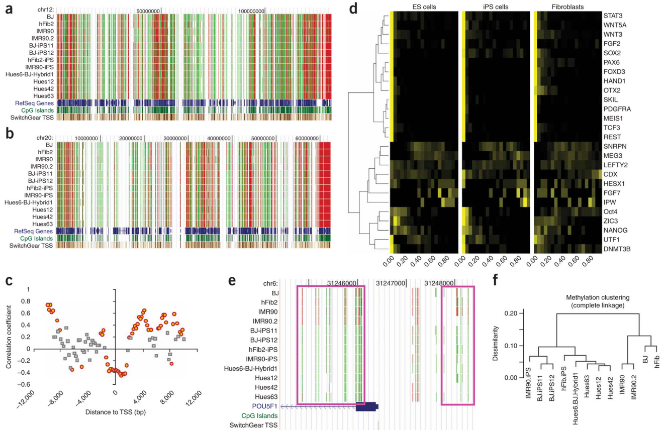
Figure 3. Patterns of CpG methylation in fibroblasts and pluripotent cells. (a,b) Patterns of CpG island methylation on chromosomes 12 and 20 in twelve samples. Red indicates highly methylated CpG, and green indicates weakly methylated CpG. (c) Correlation between DNA methylation and gene expression. Each circle or square represents a 500-bp window. The windows in which average methylation levels are significantly correlated ( P < 0.01 ) with gene expression are highlighted as orange circles. Gray squares indicate that the correlation is not significant. (d) Clustering of 26 selected genes based on the distribution of CpG methylation in the 4-kb TSS flanking regions. The 20 columns per cell line represent the fraction of probes within the TSS region where each probe exhibits a methylation frequency such that column header value \leq methylation frequency < column header value + 0.05. For example, unmethylated TSS regions will have the highest probe fraction in the lowest value-labeled (left) column. Roughly half of the genes (14) were close to completely unmethylated in all cell types. Five genes ( OCT4 , ZIC3 , NANOG , UTF1 , DNMT3B ) that show cell-type specific changes in methylation were grouped as a cluster. (e) Methylation pattern in the TSS flanking regions of OCT4 . Two differentially methylated regions were marked by purple rectangles. (f) Hierarchical clustering of pluripotent cells and fibroblasts. The dissimilarity matrix was calculated based on Pearson correlation coefficients.
