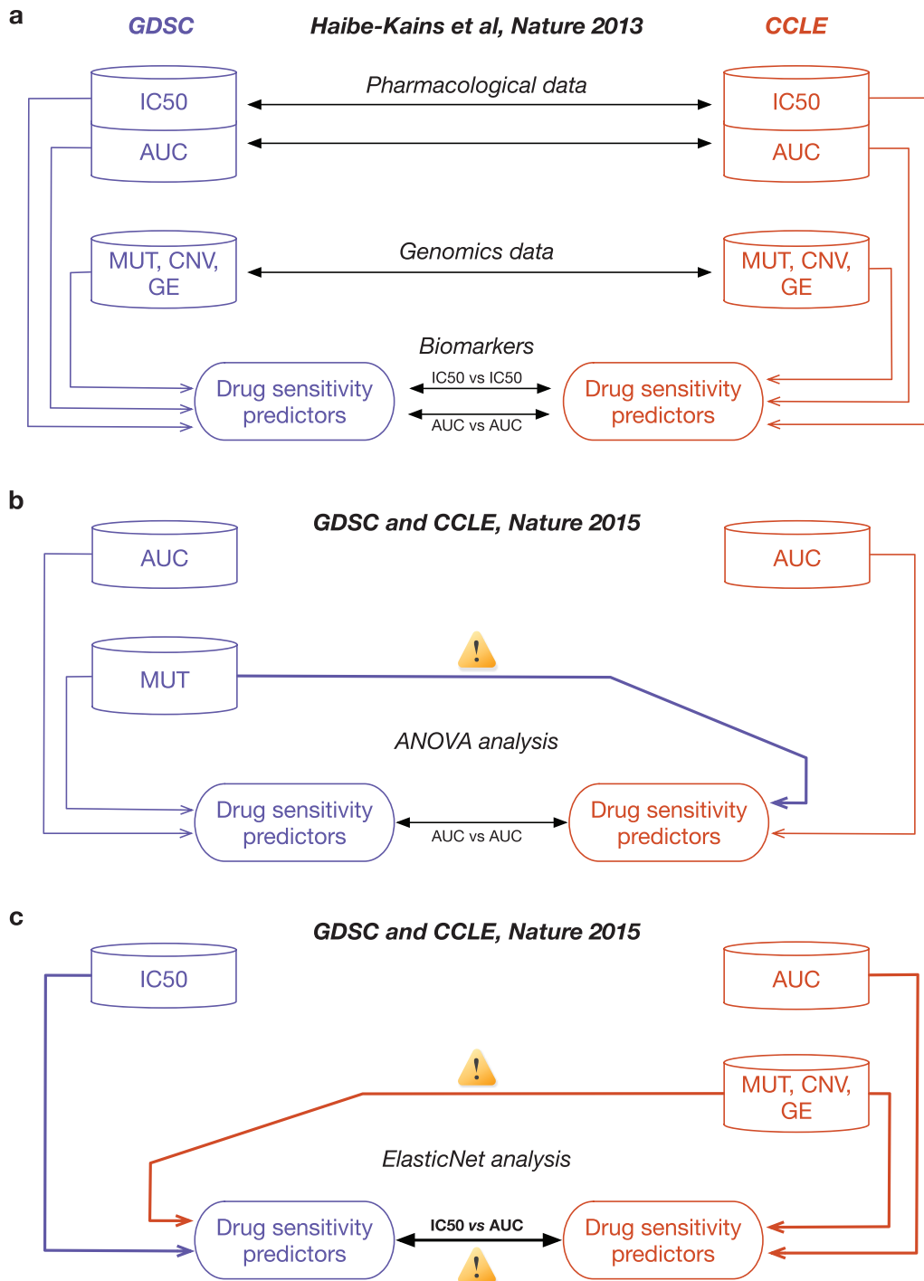
Figure 1. Analysis designs used to compare pharmacogenomic studies. (a) Analysis design used in our comparative study (Haibe-kains et al. , Nature 2013) where each data generated by GDSC and CCLE are independently compared to avoid information leak and biased assessment of consistency. (b) Analysis design used by the GDSC and CCLE investigators for their ANOVA analysis where the mutation data generated with GDSC were duplicated for use in the CCLE study. (c) Analysis design for the ElasticNet analysis where the molecular profiles from CCLE were duplicated in the GDSC study and the GDSC IC 50 were compared to CCLE AUC data. Differences between our analysis design and those used by the GDSC and CCLE investigators are indicated by yellow signs with exclamation mark symbol.
