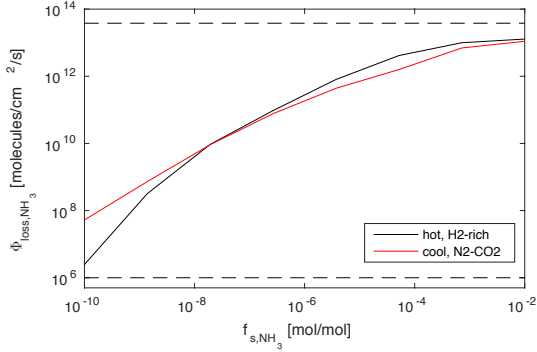
Figure 3: Predicted ammonia destruction rates as a function of surface \text{NH}_3 molar concentration. The black and red lines show results from the photochemical code for a hot hydrogen-rich atmosphere ( f_{\text{H}_2} = 0.5 mol/mol, f_{\text{N}_2} = 0.5 mol/mol, T_s = 700 K, p_s = 30 bar) with constant eddy diffusion \kappa_D = 10^5 \text{cm}^2 \text{s}^{-1} and a cool \text{N}_2 - \text{CO}_2 atmosphere ( f_{\text{N}_2} = 0.9 mol/mol, f_{\text{CO}_2} = 0.1 mol/mol, T_s = 300 K, p_s = 1 bar) with present-day eddy diffusion profile, respectively. The dashed lines show the upper and lower limits for photolysis rates derived from the results.
