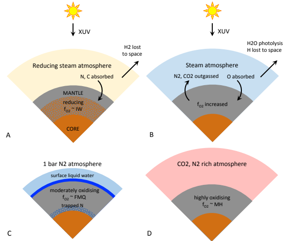
Figure 5: Schematic of the water loss redox pump explanation for the differing atmospheric \text{N}_2 inventories of Earth and Venus. Both planets start in state A. Earth evolves directly to state C, whereas Venus passes through state B before ending up in D. See text for full description.
