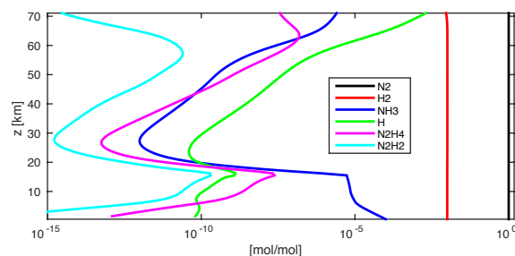
Figure 2: Example results from the photochemical model. Steady state atmospheric molar concentrations of major species for a N_2 -dominated atmosphere with T_s = 300 K, p_s = 1 bar, 10^4 ppmv H_2 , surface NH_3 concentration of 100 ppmv, and eddy diffusion and rain-out included based on present-day parametrizations.
