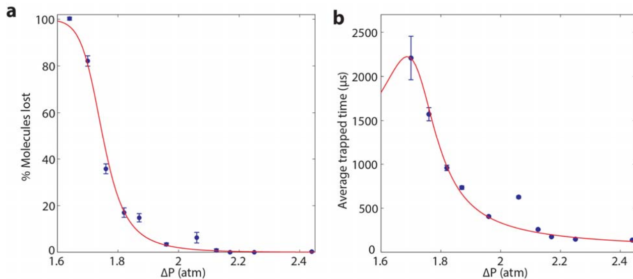
Figure 4. (a) Percentage of unsuccessful translocations at different pressures. The solid line is the prediction of the model in the text. (b) Average escape time of molecules in the P-V trap, for successful translocations only. The solid line is the prediction of the model in the text.
