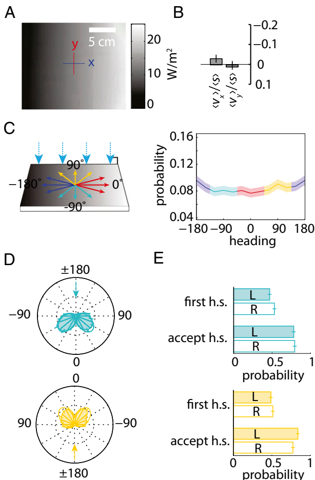
Fig. 4. Larvae do not phototax on a shallow linear spatial gradient. (A) Irradiance map of the linear gradient lightscape. (B) Canton-S larvae navigational index, \langle v \rangle / \langle s \rangle , computed for x and y directions on the linear gradient lightscape. n = 15 animals, 128 experiments. (C) (Left) Schematic of the linear gradient lightscape. Light is incident to plate at 90^\circ . (Right) Probability of orientation vs. heading in runs for the linear gradient lightscape. The shaded area around the curve represents SEM. (D) Polar histograms of heading changes achieved by turns for a fixed initial run heading before turn. The arrow indicates the initial heading. (E) Probability of first head-sweep (h.s.) direction and head-sweep acceptance to left (L) and right (R) sorted by initial heading for linear gradient lightscape.
