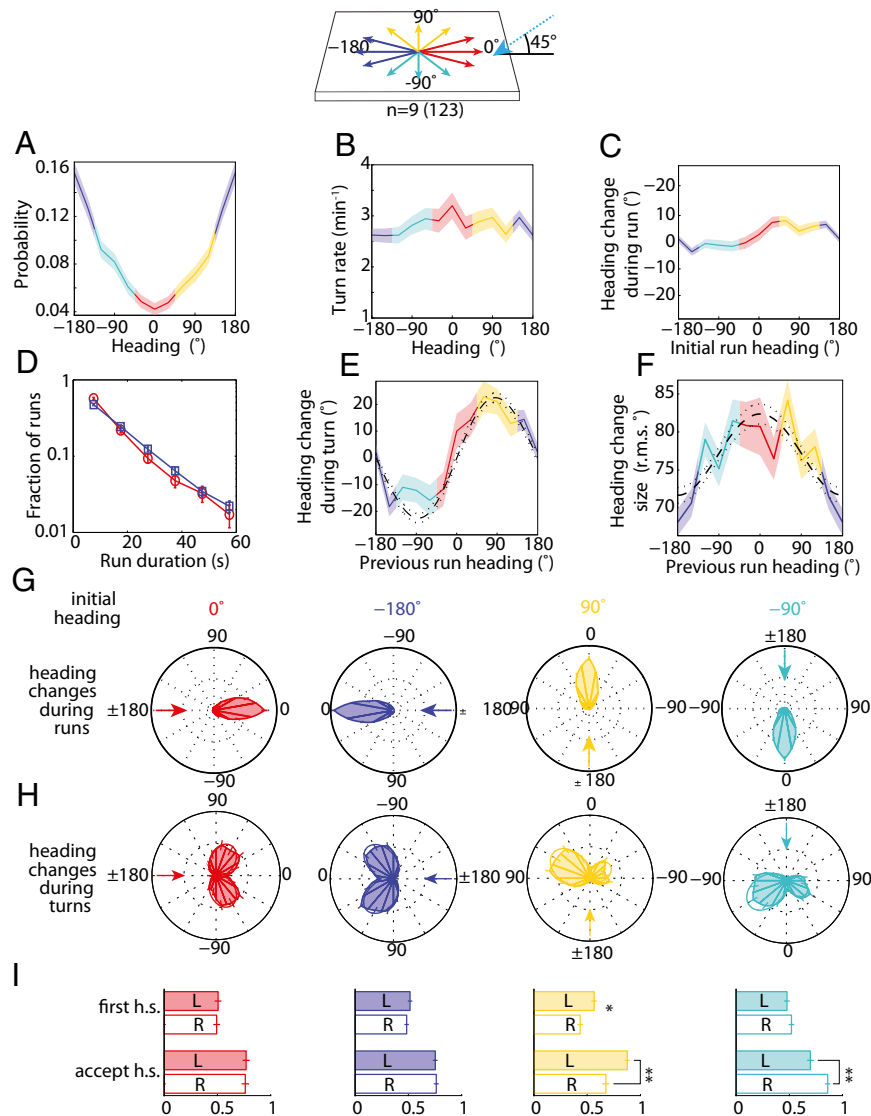
Fig. 7. Directional lightscapes navigational strategy. (Top) Schematic of headings on the directional lightscape. (A) Probability of heading during runs. (B) Turn rate vs. heading in run. (C) Mean heading change achieved in run vs. heading in initial run. (D) Distribution of run lengths for larval headings into incident light rays (red, 0^\circ , nonpreferred heading) and away from incident light rays (blue, 180^\circ , preferred heading). (E) Mean heading change during turn vs. previous run heading. Dashed and dotted lines are the prediction and 95% confidence interval of a model with biases in turn magnitude and head-swing acceptance (11). (F) Heading change size (rms degrees) vs. initial heading (in degrees). Dashed and dotted lines are the prediction and 95% confidence interval of the model as described in E. (G) Polar histograms of heading changes achieved by runs for fixed initial heading, indicated by arrow. (H) Polar histograms of heading changes achieved by turns for a fixed initial heading before turn. The arrow indicates the initial heading. (I) Probability of first head-sweep (h.s.) direction and acceptance of head-sweeps, whether left (L) or right (R), sorted by initial heading. In A–F, shaded areas represent SEM. In I, * indicates P < 0.01 and ** indicates P < 0.0001 using binomial statistics. Data represent nine experiments and 123 animals.
