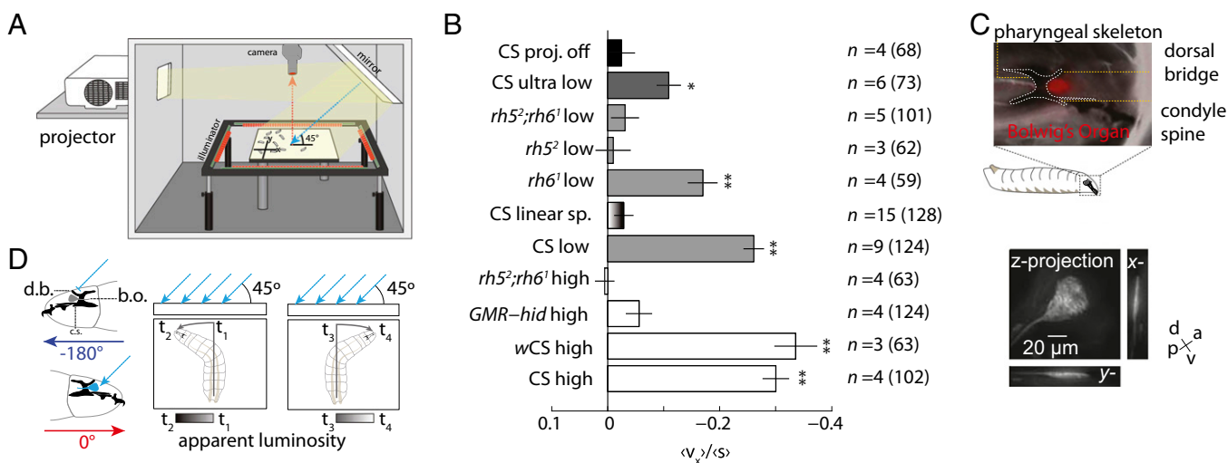
Fig. 6. Directional lightscape navigation requires the Rh5 PRs of the BO. (A) Schematic of directional lightscape apparatus. Light rays are incident to larvae at 45^\circ . (B) Navigational index ( \langle v_x \rangle / \langle s \rangle ). Rejection of null hypothesis that dataset has same mean as projector-off dataset: * P < 0.01 , ** P < 0.0001 , Welch two-tailed t test. For light intensities see Figs. S1 and S2. n = number experiments (number larvae). (C) The BO sits in a pigment cup formed by the cephalopharyngeal skeleton. (Upper) Fluorescence microscopy of GMR-RFP merged with bright-field microscopy. The white dotted line indicates the cephalopharyngeal skeleton. (Lower) Maximum intensity projections from 3D confocal microscopy of the BO in longGMR > CDB::GFP larva. (D) Schematic of differential view angle of the BO conferred by cephalopharyngeal skeleton.
