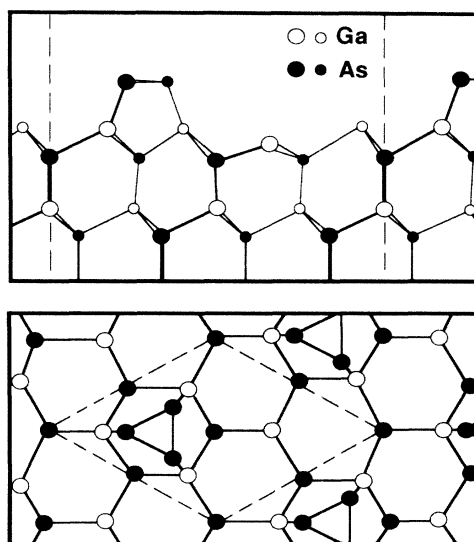
FIG. 2. Upper panel: Side view [(110) plane] of the GaAs(111)2×2 surface As triangle model. Larger size atoms are in the plane of the paper. Smaller size atoms are in a parallel plane. Lower panel: Top view of the As-triangle model. Dashed lines indicate a 2×2 unit cell.
