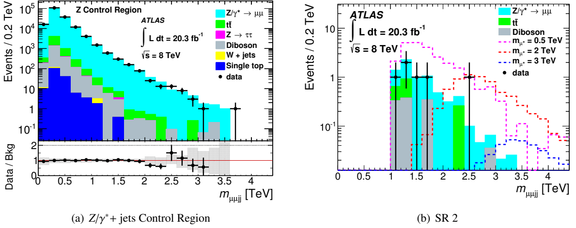
Figure 2: The \mu\mu jj mass distribution for (a) the Z/\gamma^* + jets control region with the MC predictions and (b) for SR 2 ( m_{\mu\mu} > 550 GeV, S_T > 900 GeV, and m_{\mu\mu jj} > 1000 GeV) with three representative signal distributions for \mu^* masses of 500, 2000, and 3000 GeV and for \Lambda = 5 TeV. The background expectations are determined after the fit, and the grey band on the ratio plot in (a) gives the systematic uncertainty. For (b) there are no expected events from the single top, W + jets, and Z \rightarrow \tau\tau processes. SR 2 is not the most sensitive signal region for the latter two m_{\mu^*} masses. They are shown for comparison.
