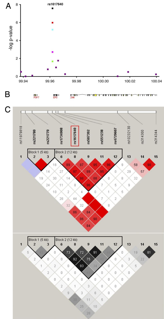
Fig. 1. Genetic association. (A) Negative log P values (y axis) from association analyses for 11 SNPs in the chromosome 7q22 region harboring the EPO gene (see also Table S3). The violet squares represent all SNPs around rs1617640 from the Utah T2D cohort. The green square represents rs1617640 from the Boston T1D cohort. The pink square represents rs1617640 from the Utah T2D cohort. The light blue square represents rs1617640 from the GoKinD patients who have retinopathy and nephropathy but have not progressed into ESRD. The red square represents rs1617640 from the GoKinD patients who have both PDR and ESRD. The black square represents rs1617640 from the GoKinD cohort. (B) Genomic structure and locations of genes between base pairs 99.94 and 100.04 million (National Center for Biotechnology Information build 35). (C) Pairwise D' and R 2 Haploview (38) plots for SNPs in chromosome 7 in the region around the EPO gene when Utah T2D case and control data are used.
