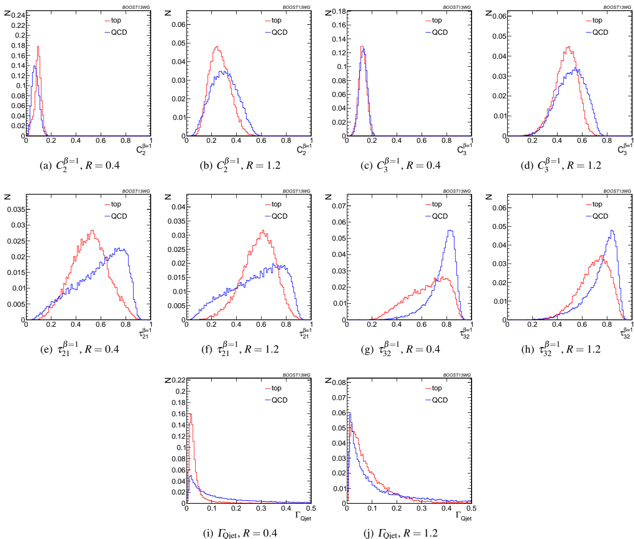
Fig. 36 Comparison of various shape variables in the p_T = 1.5-1.6 TeV bin and different values of the anti- k_T radius R .
