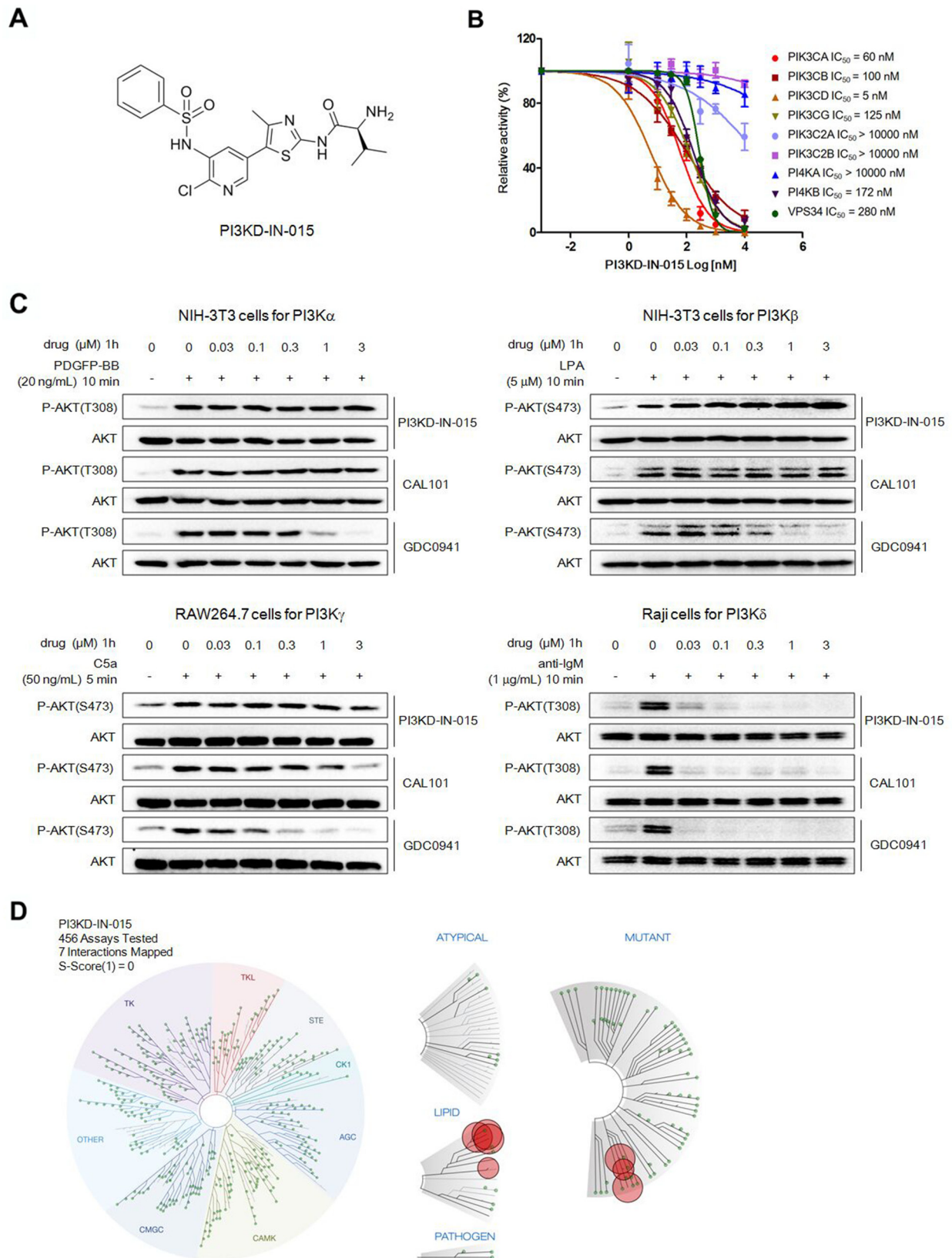
Figure 1: Discovery of PI3KD-IN-015 as a potent and selective PI3K \delta inhibitor A. Chemical Structure of PI3KD-IN-015. B. ADP-glo biochemical assay determination of IC_{50} of PI3KD-IN-015 against different PI3K isoforms. C. Determination of PI3KD-IN-015 inhibitory activities against PI3K \alpha , \beta , \delta and \gamma in cellular background. D. TreeSpot™ demonstration of PI3KD-IN-015 selectivity against a panel of 456 kinases with DiscoverX KinomeScan™ technology with an S (1) score = 0.
