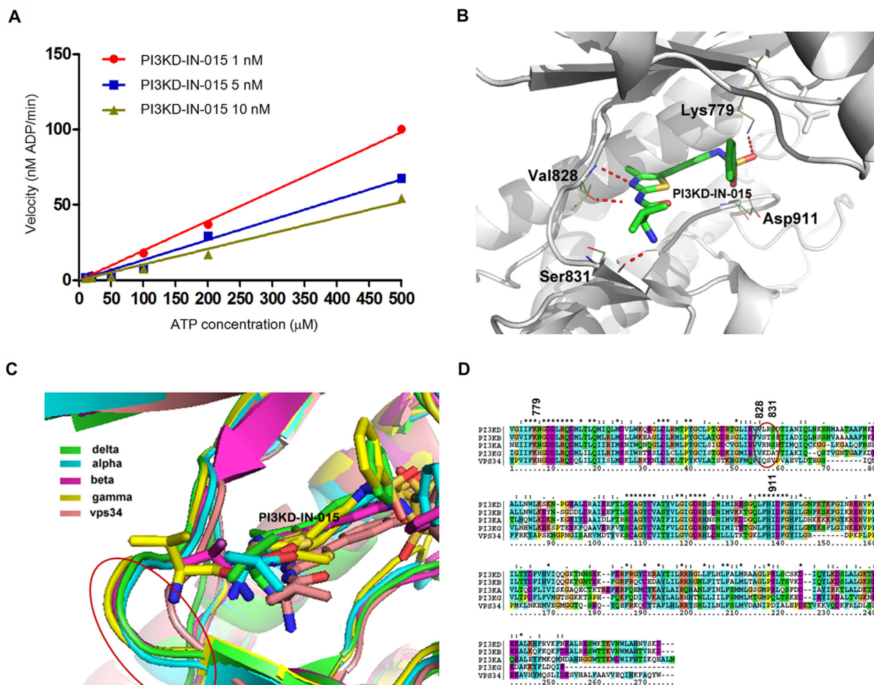
Figure 2: Structural basis for PI3KD-IN-015's selectivity among PI3K isoforms A. ATP competitive kinetic study of PI3KD-IN-015 against PI3K \delta . B. PI3KD-IN-015 was docked into PI3K \delta (homology model, template PDB ID: 2WXF). C. Superimposition of PI3KD-IN-015 in complex with PI3K \alpha , \beta , \delta , \gamma and vps34. D. Sequence alignment of PI3K \alpha , \beta , \delta , \gamma and vps34 kinase domain.
